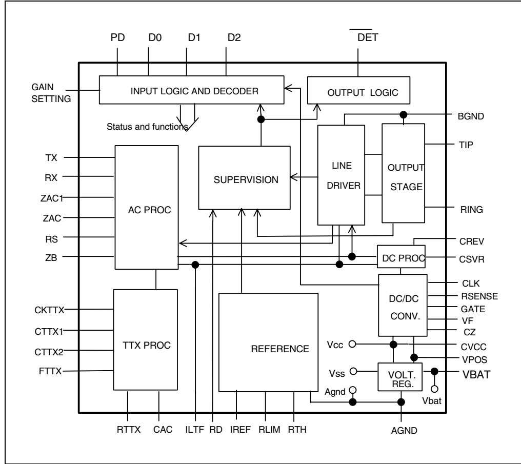
Figure 1. Block diagram
