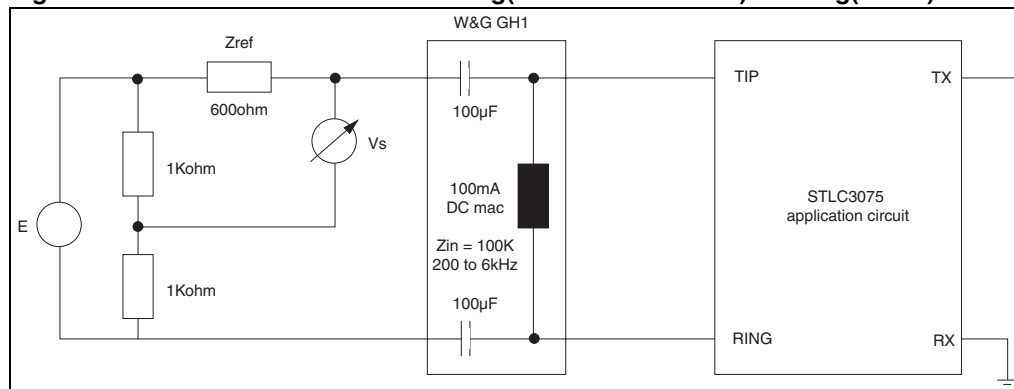
Figure 12. 2W return loss 2WRL = 20\text{Log}(|Z_{ref} + Z_s|/|Z_{ref} - Z_s|) = 20\text{Log}(E/2V_s)
