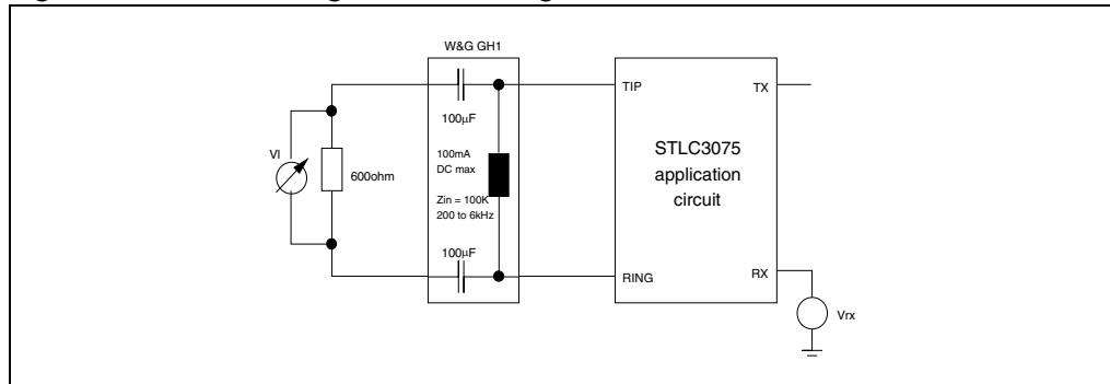
Figure 15. G42 receive gain G_{42} = 20\text{Log}|V_i/V_{rx}|
