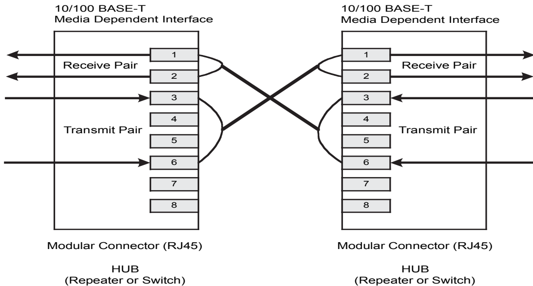
Figure 2. Crossover Cable
