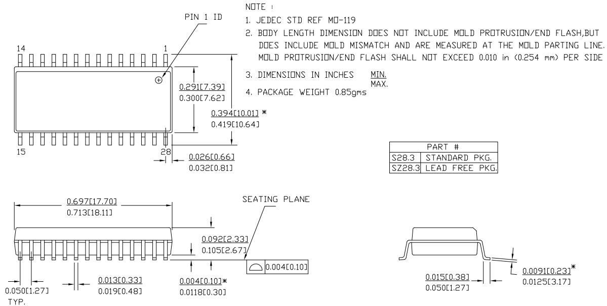
Figure 14. 28-Pin (300-Mil) Molded SOIC S21
