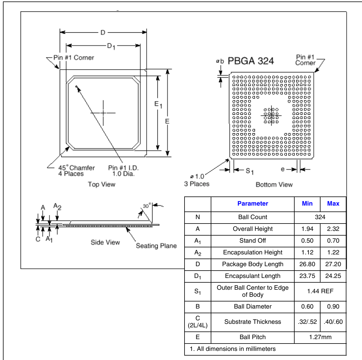
Figure 28. Package Specifications
