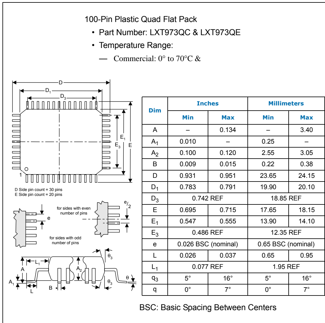
Figure 43 Mechanical Specifications
