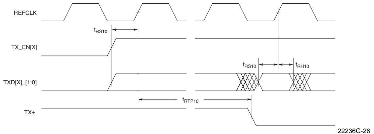
Figure 24. RMII 10 Mbps Transmit Start of Packet
