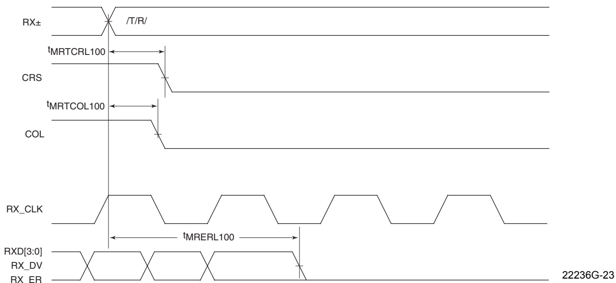
Figure 21. 100 Mbps MII Receive End of Packet Timing
