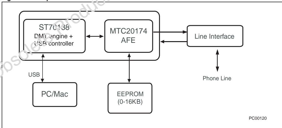
Figure 1. Chipset architecture overview
