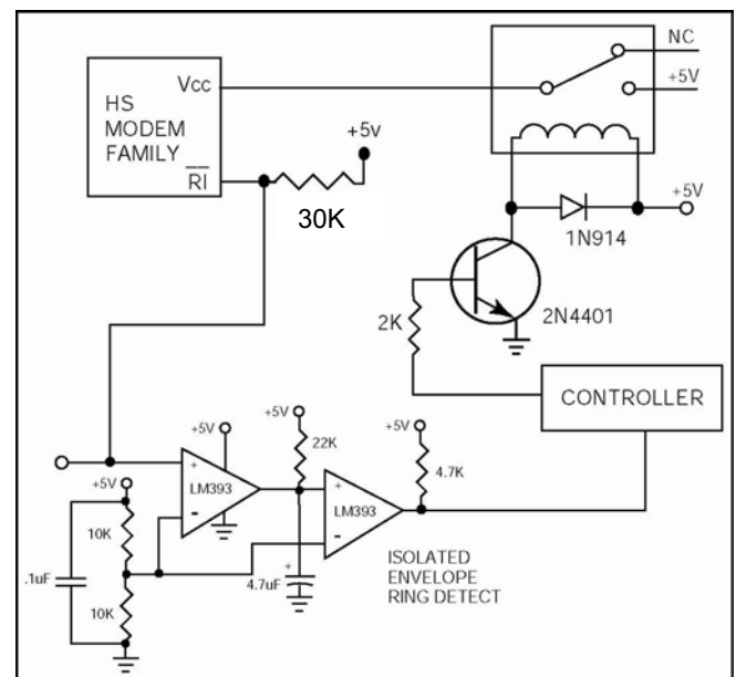
Figure 3. Example of Zero Power Operation.
