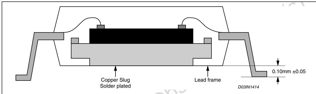
Figure 28. Soldering Information
