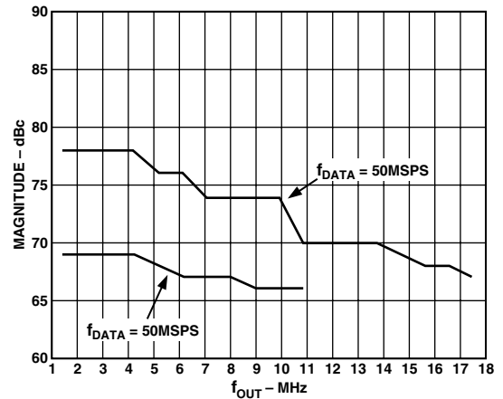
TPC 10. "Out of Band" SFDR vs. f_{OUT} @ f_{DATA} = 32 \text{ MSPS} and 50 \text{ MSPS}
