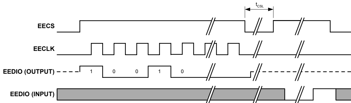
Figure 3.13 EEPROM ERALL Cycle
