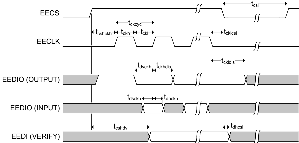
Figure 6.8 EEPROM Timing
