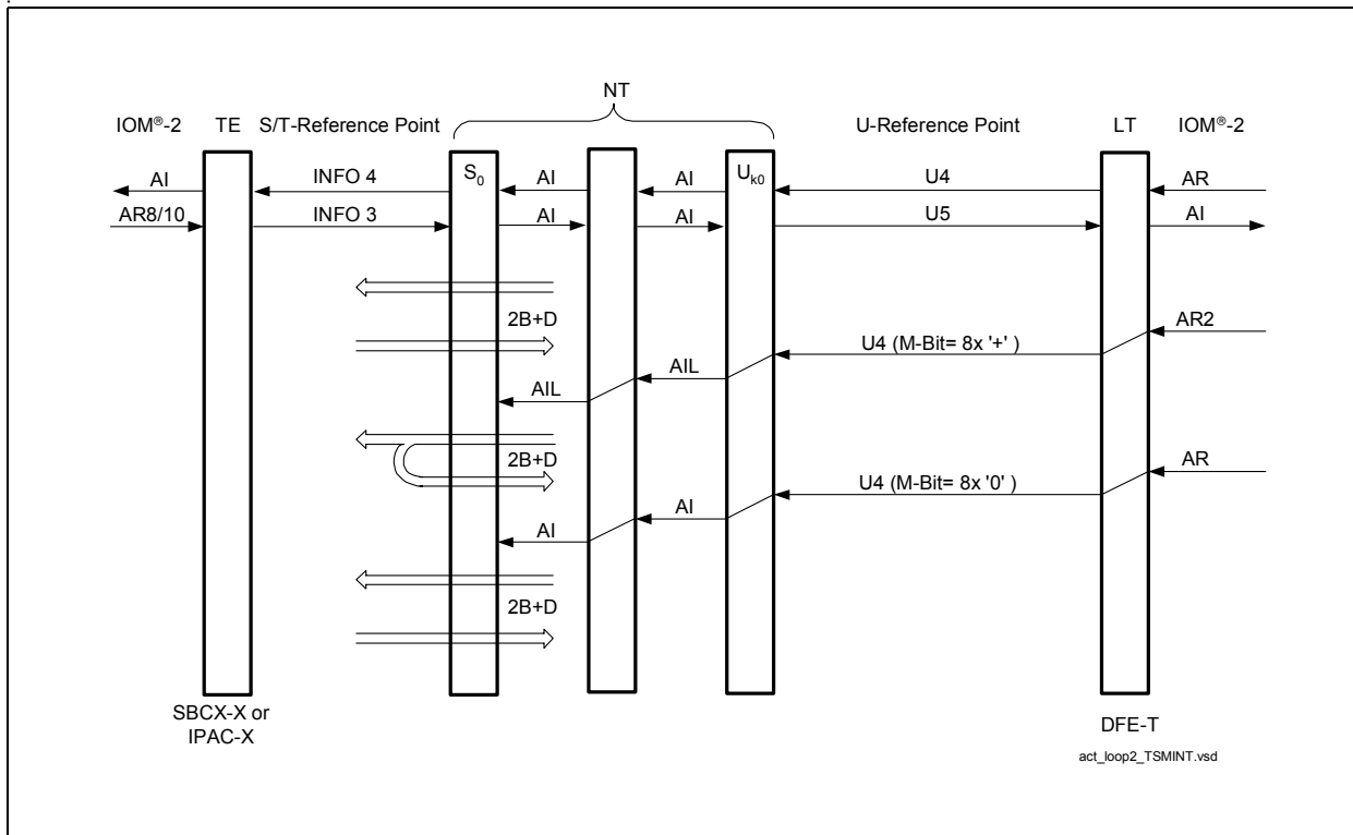
Figure 57 Loop 2
