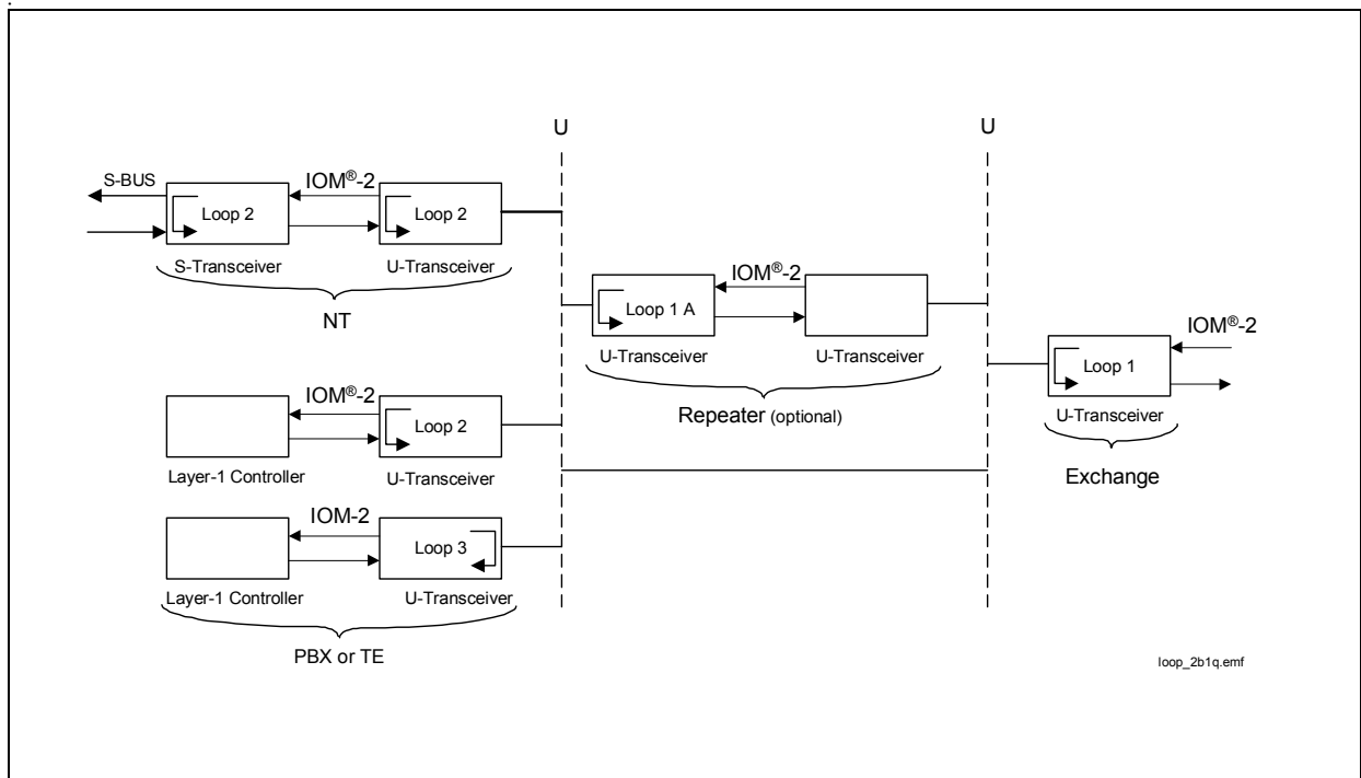
Figure 58 Test Loopbacks
