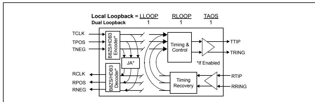
Figure 12 Dual Loopback
