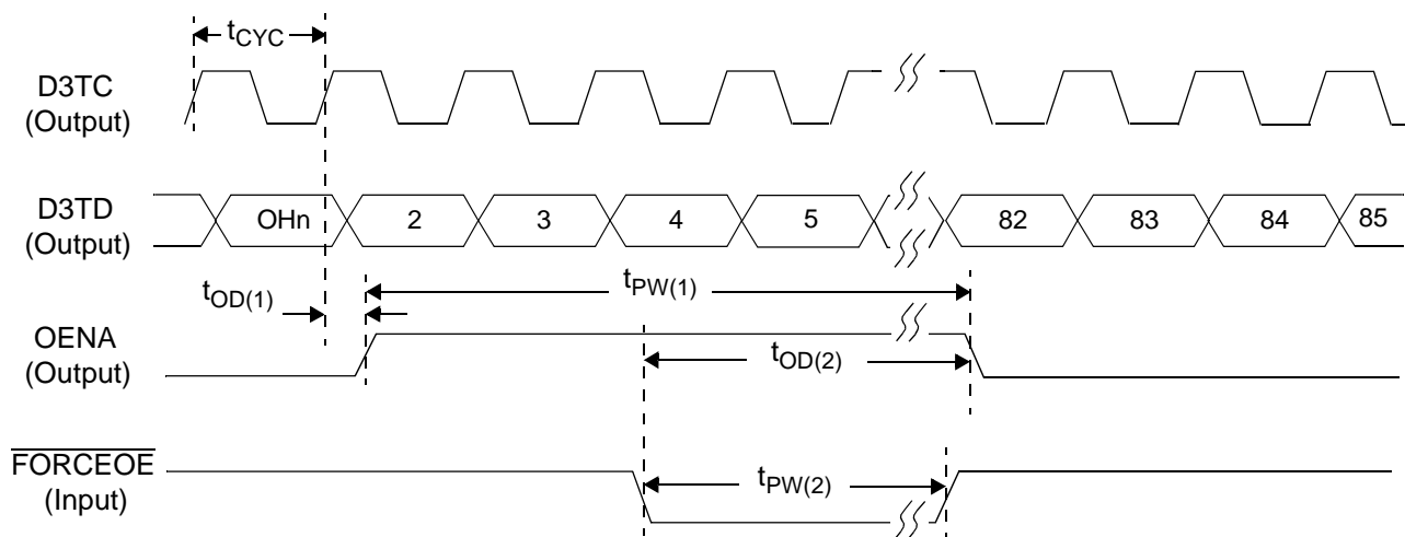
Figure 14. Force Overhead Bit Error Timing
