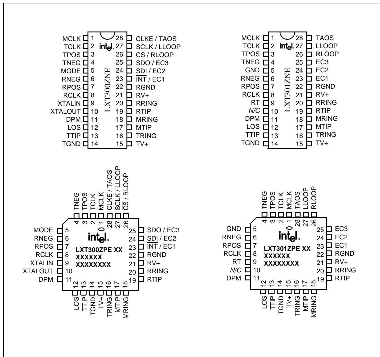
Figure 2. LXT300 Pin Assignments and Package Markings
