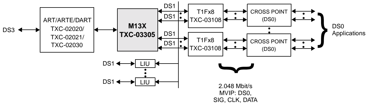
Figure 26. Example Channelized T3 Application
