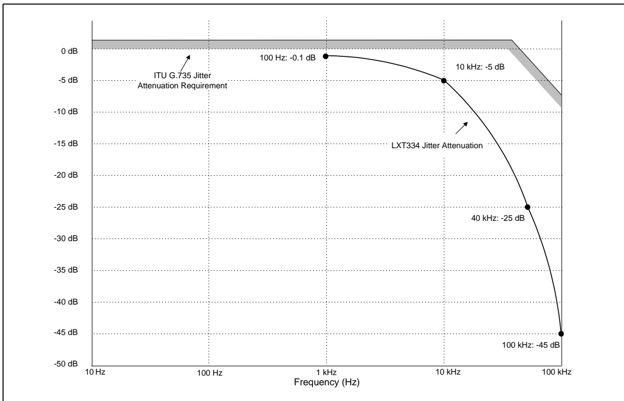
Figure 19. Jitter Attenuation—G.735
