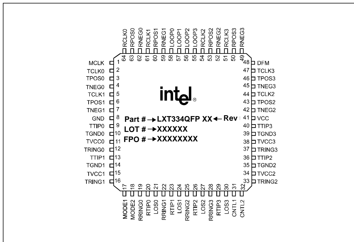
Figure 2. LXT334 64 Pin Assignments and Markings
