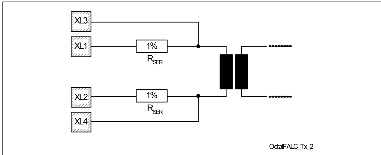
Figure 29 Transmit Impedances
