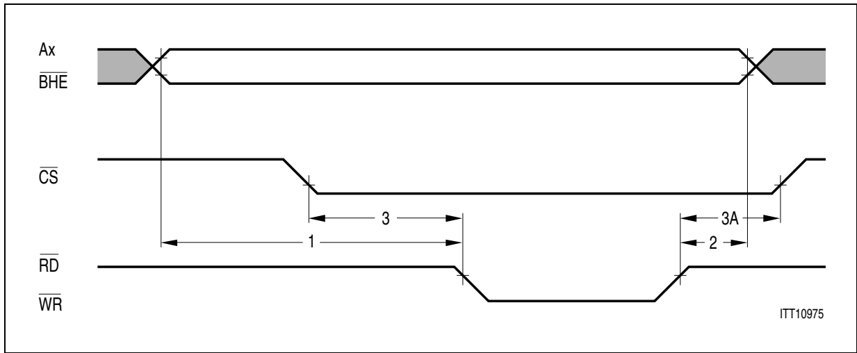
Figure 6 Intel Non Multiplexed Address Timing
