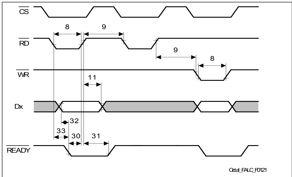
Figure 3 Intel Read Cycle Timing
