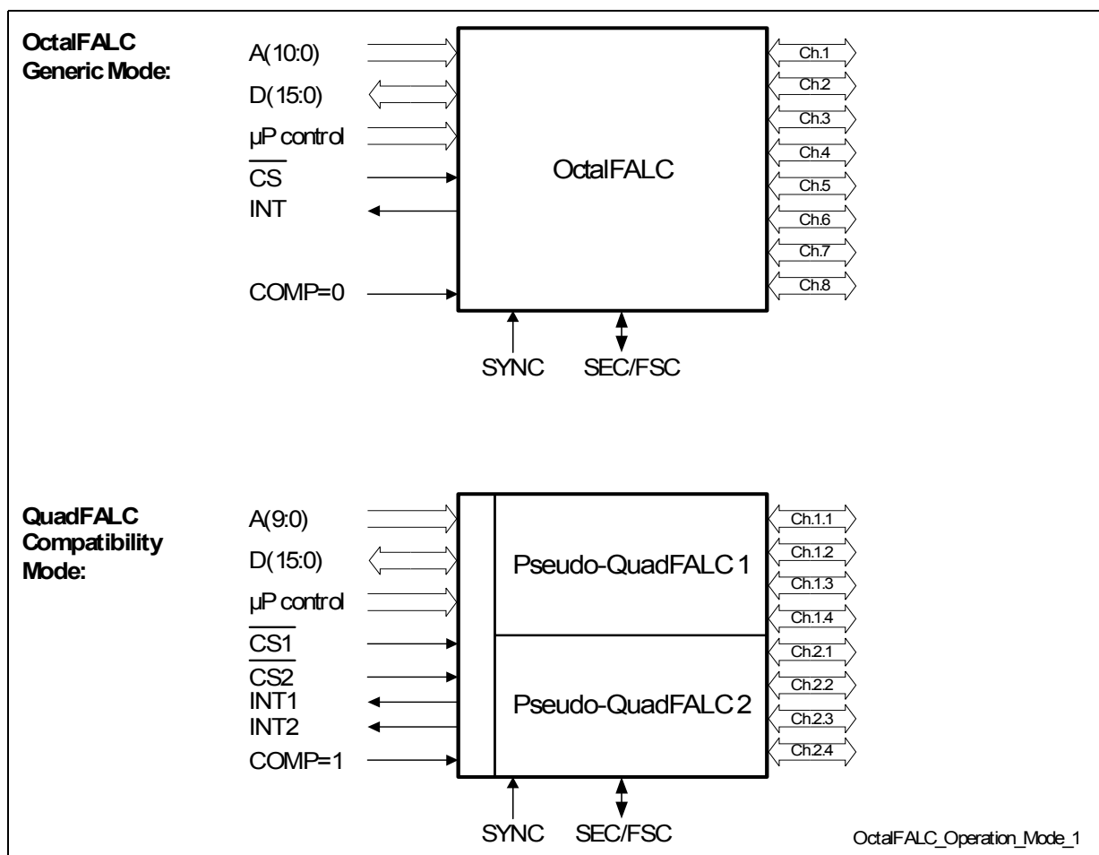
Figure 2 Basic Operation Modes for Microcontroller interface
