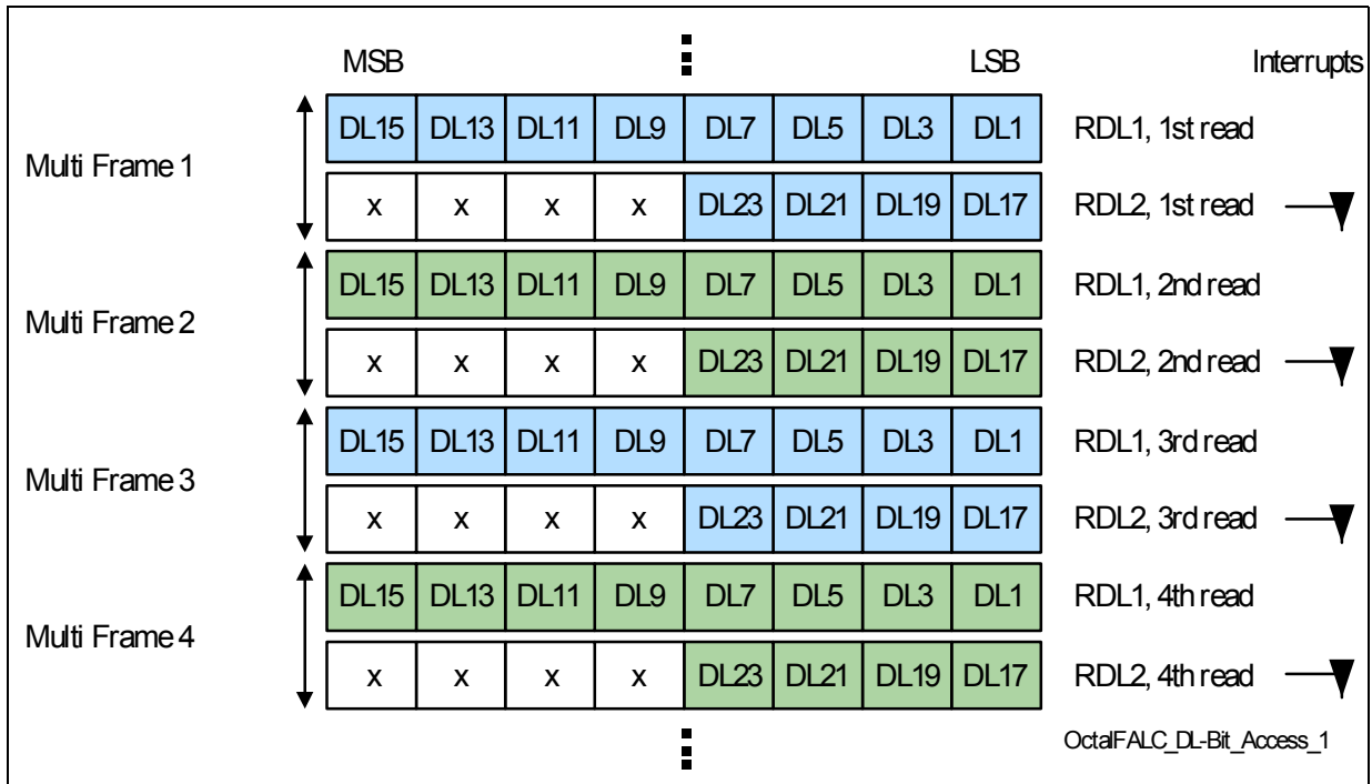
Figure 22 Standard DL-Bit Access in ESF Mode
