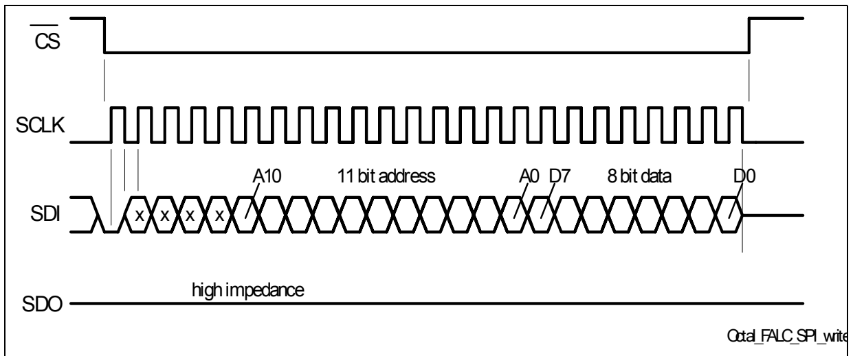
Figure 16 SPI Write Operation
