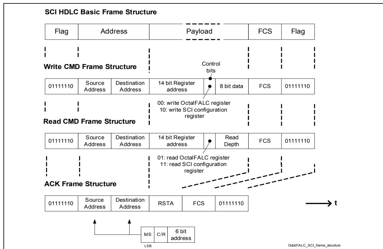
Figure 12 Frame Structure of OctalFALC™ SCI Messages
