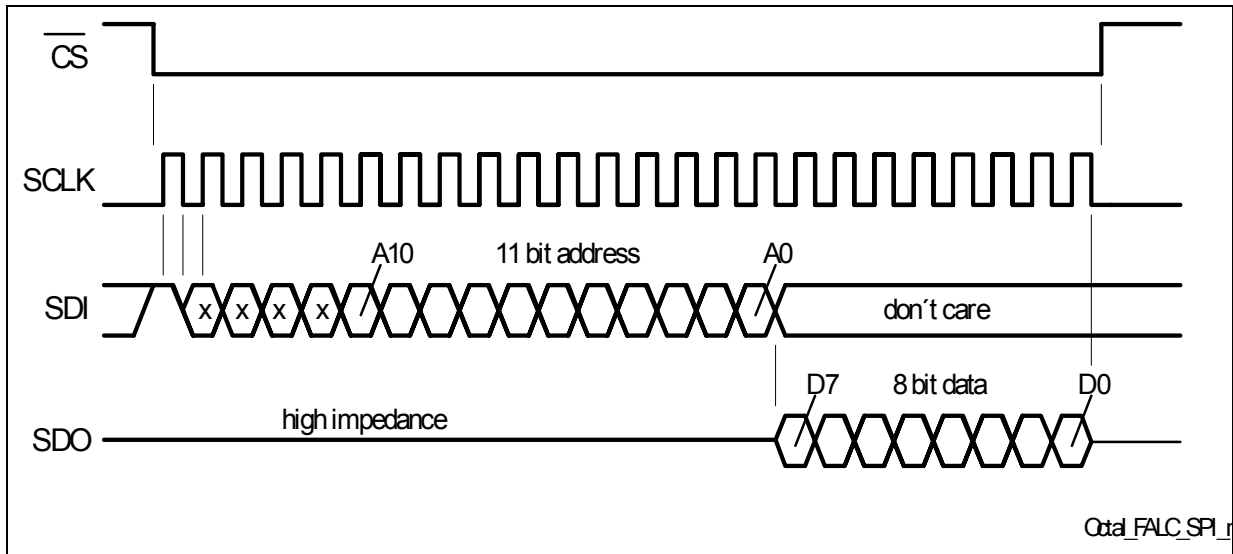
Figure 15 SPI Read Operation
