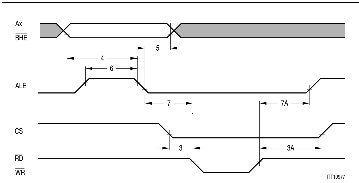
Figure 5 Intel Multiplexed Address Timing
