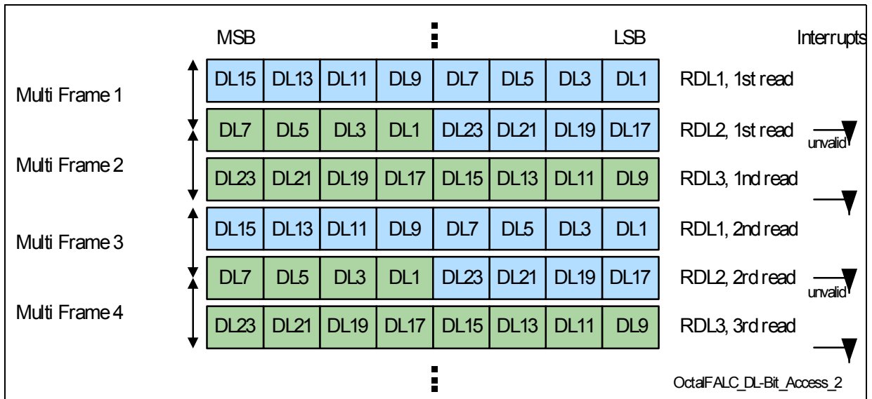
Figure 23 Optional DL-Bit Access in ESF Mode
