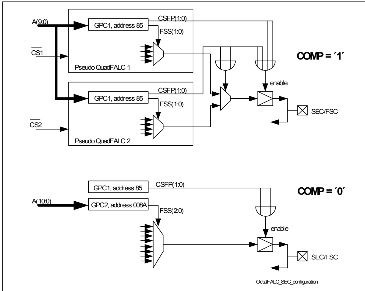
Figure 33 Principle of configuration of SEC/FSC Output
