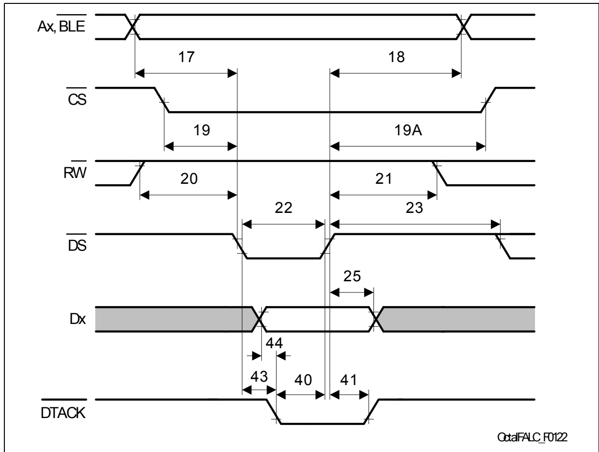
Figure 7 Motorola Read Cycle Timing
