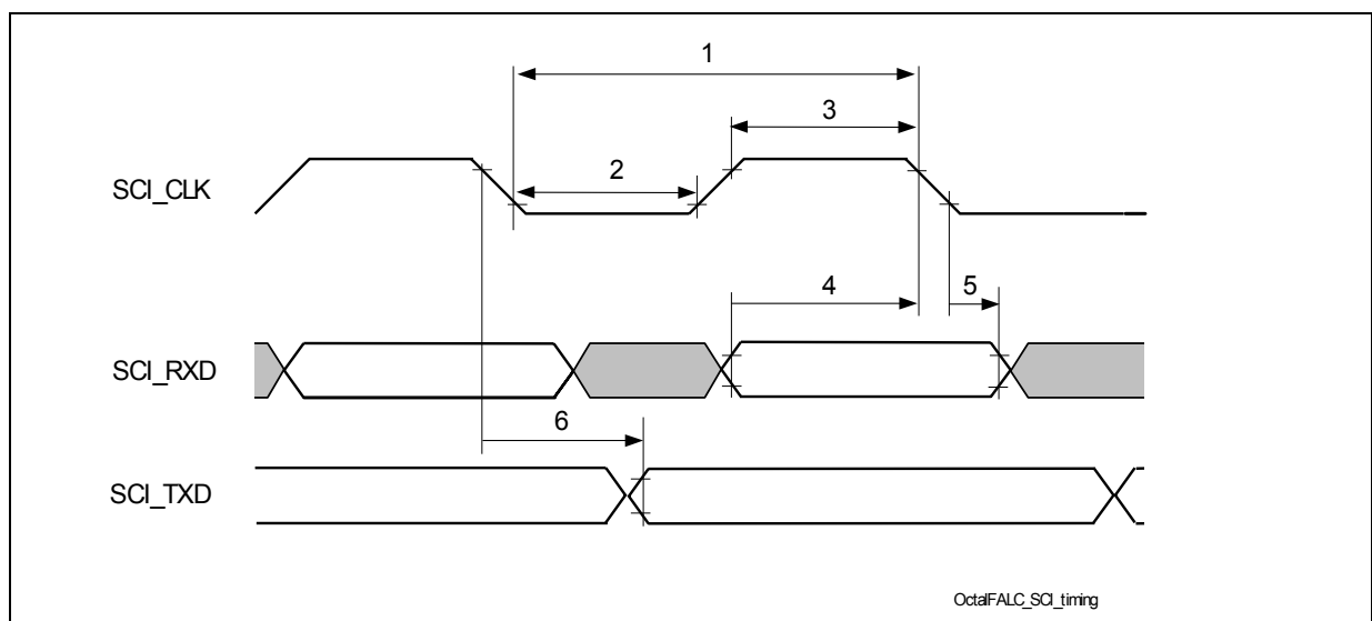
Figure 14 SCI Interface Timing
