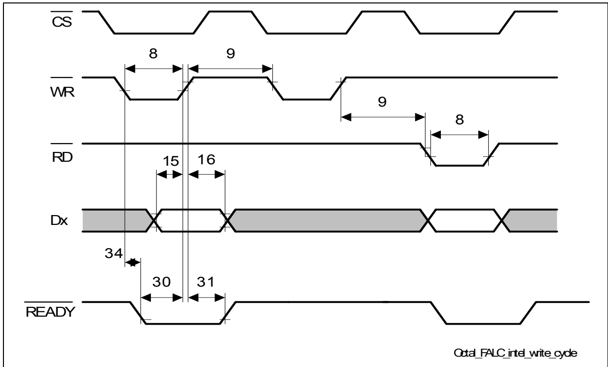
Figure 4 Intel Write Cycle Timing
