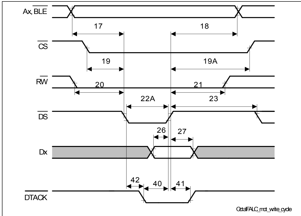
Figure 8 Motorola Write Cycle Timing
