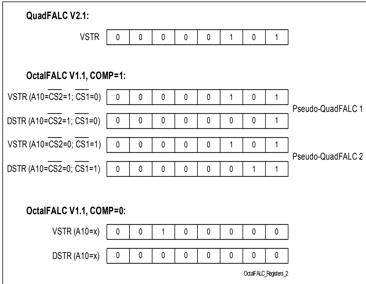
Figure 32 VSTR and DSTR Register Compatibility
