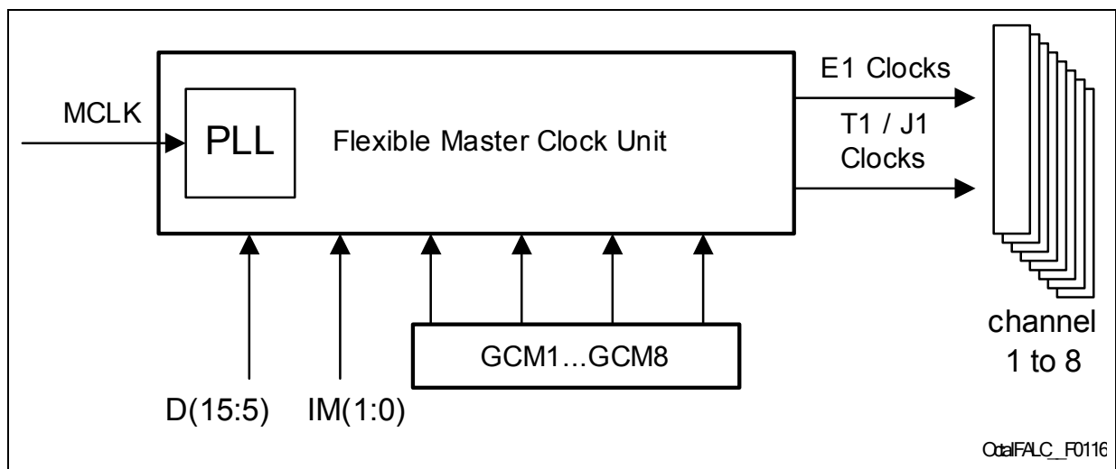
Figure 20 Flexible Master Clock Unit
