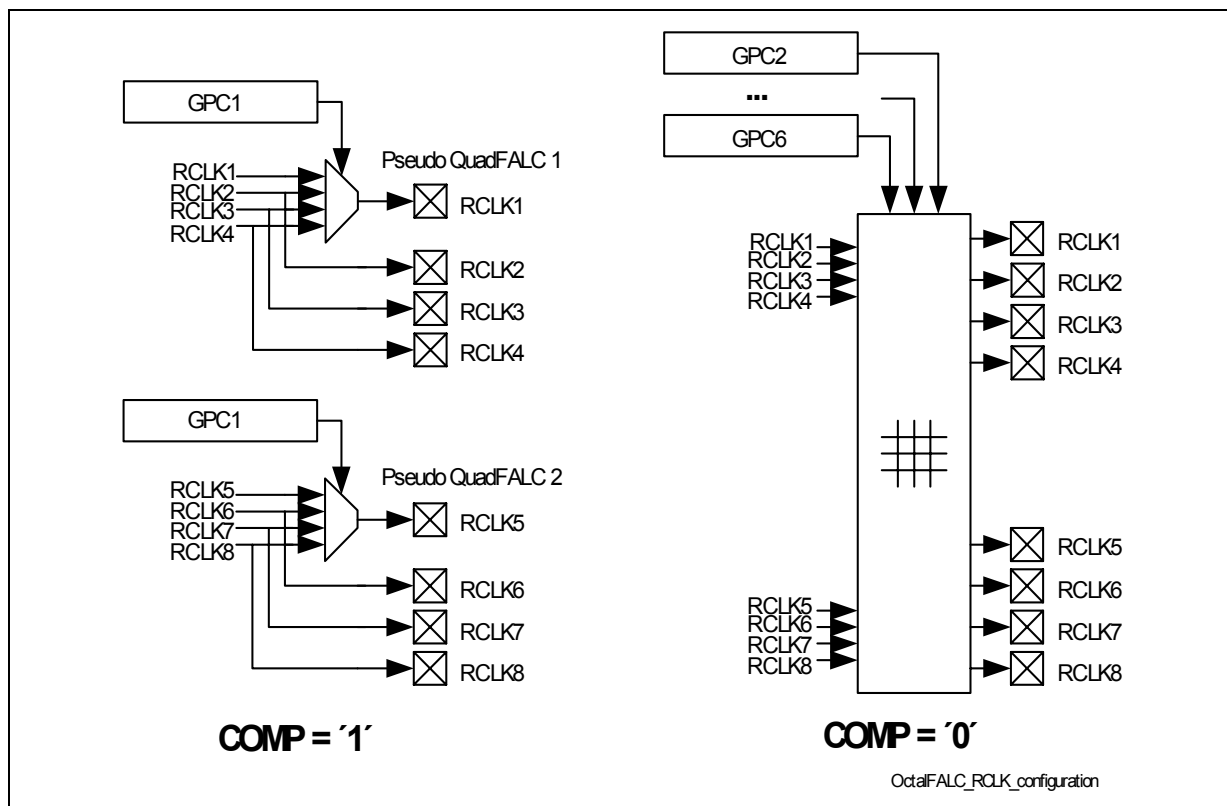
Figure 18 Receive Clock Selection
