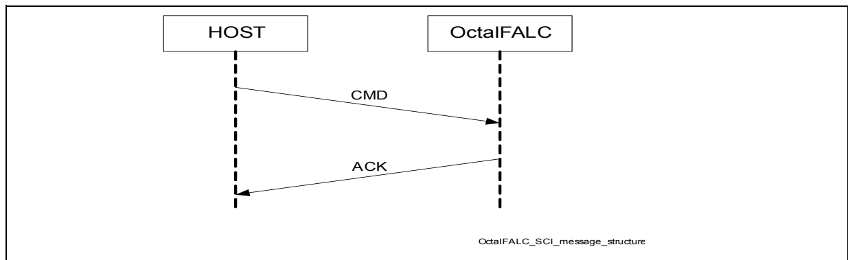
Figure 11 SCI Message Structure of OctalFALC™
