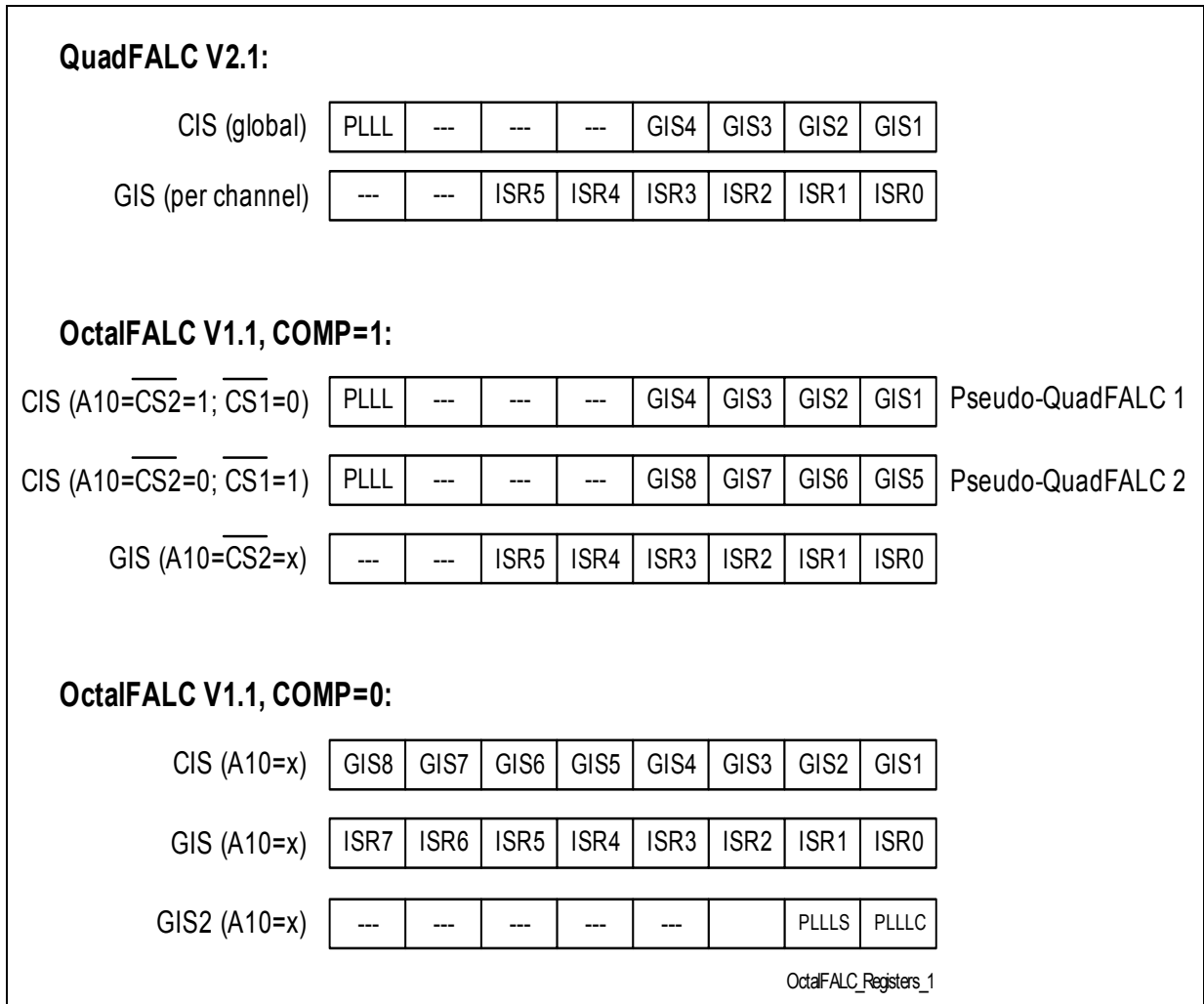
Figure 31 GIS Register Compatibility
