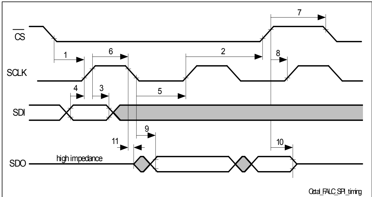
Figure 17 SPI Interface Timing
