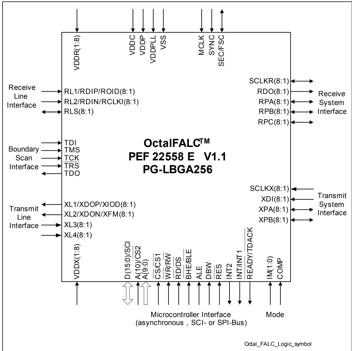
Figure 1 Logic Symbol
