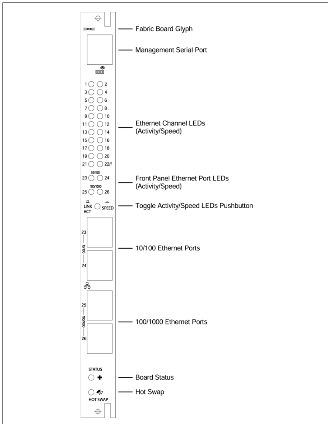
Figure 3. Front Panel
