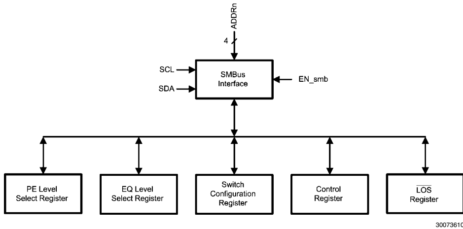
FIGURE 10. DS25CP104A Registers Block Diagram
