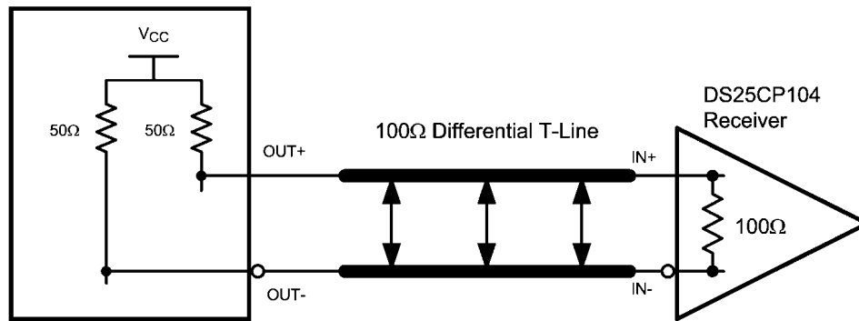
Typical CML Driver DC-Coupled Interface to DS25CP104A Input
