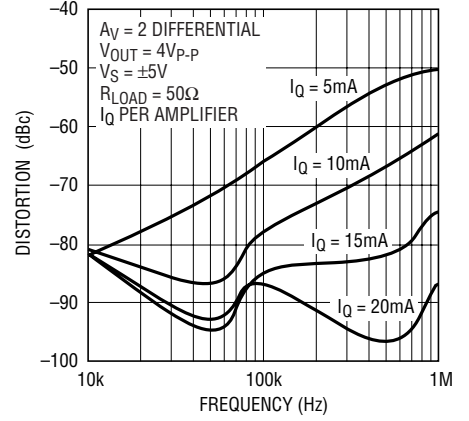
LT1795 G18
