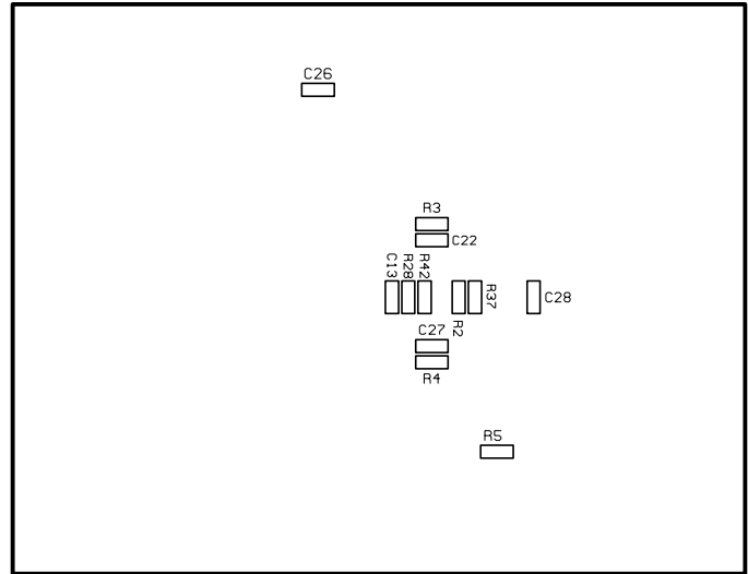
Figure 18. Assembly Bottom
