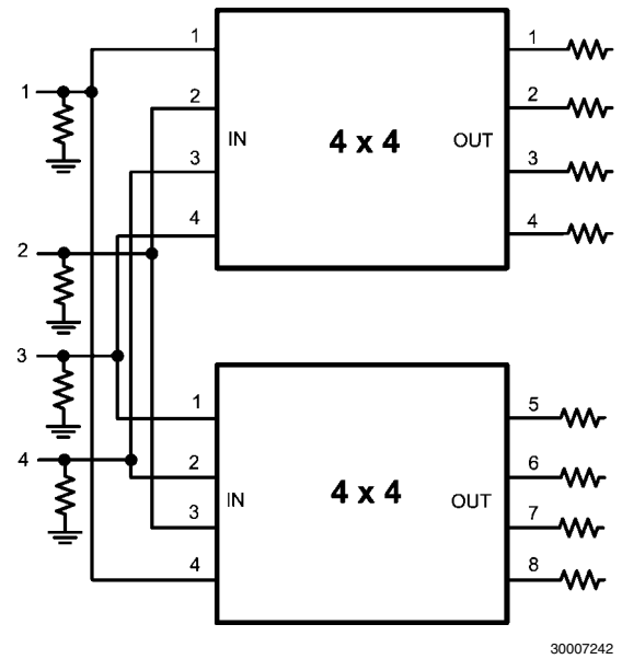
FIGURE 1. Output Expansion
