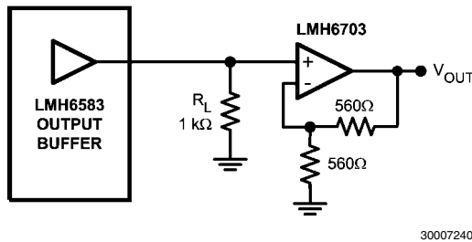
FIGURE 6. Buffered Output
