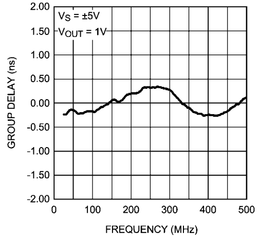
Group Delay
