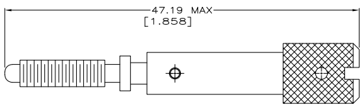
ASSEMBLED VIEW
