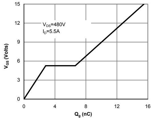
Figure 8: Gate-Charge Characteristics
