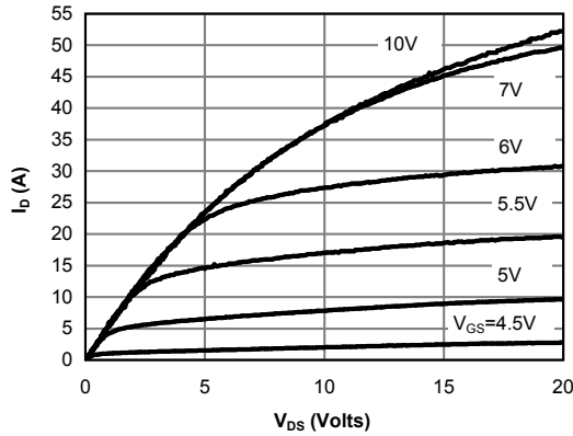
Figure 1: On-Region Characteristics@25°C
