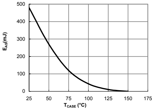
Figure 13: Avalanche energy
