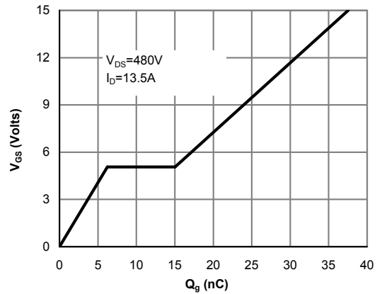
Figure 8: Gate-Charge Characteristics
