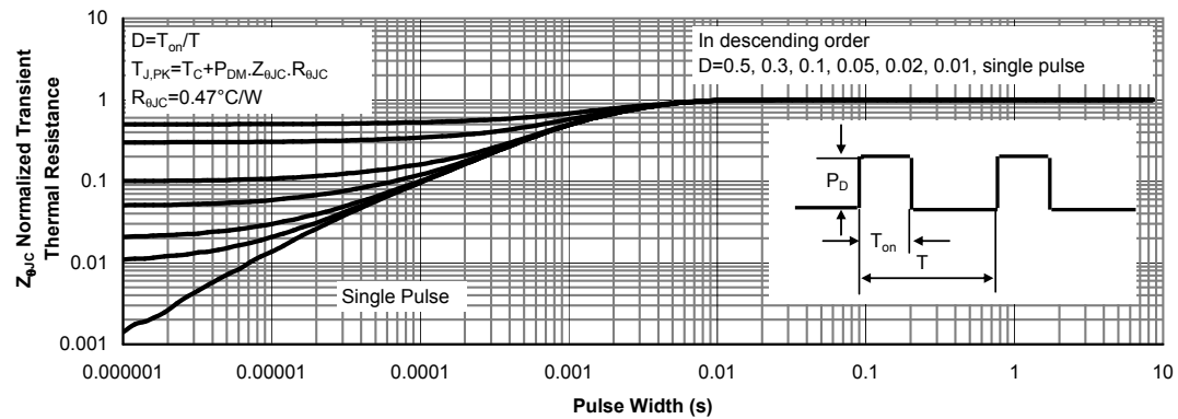
Figure 15: Normalized Maximum Transient Thermal Impedance for AOT(B)20S60 (Note F)
