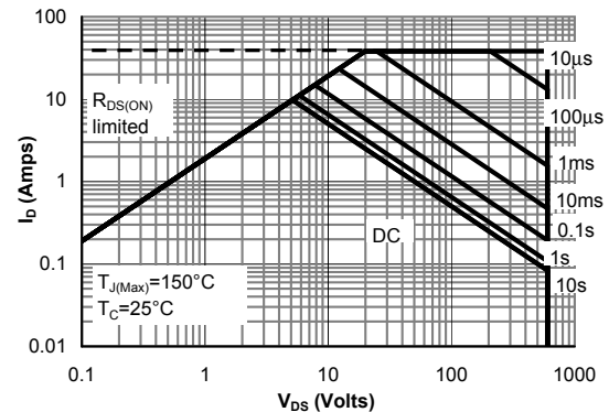
Figure 12: Maximum Forward Biased Safe Operating Area for AOTF20S60 (Note F)
