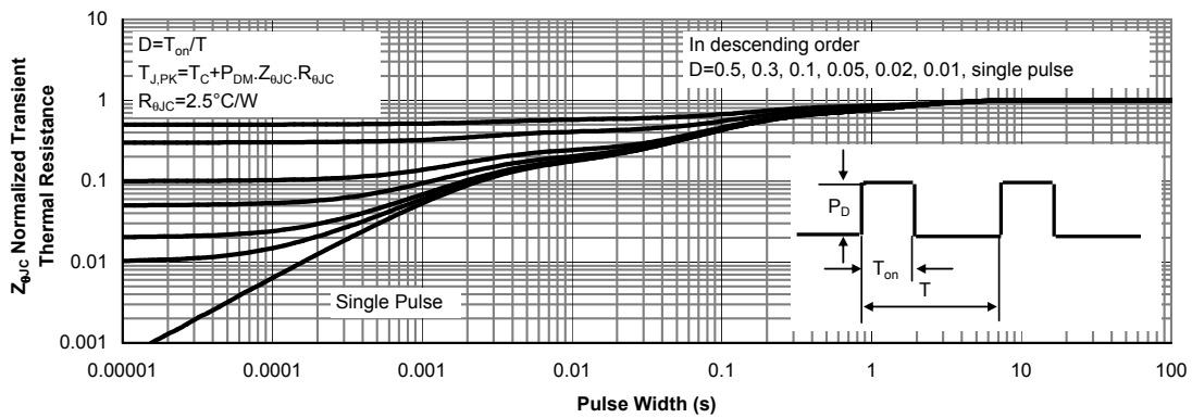
Figure 16: Normalized Maximum Transient Thermal Impedance for AOTF20S60 (Note F)
