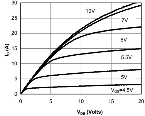
Figure 2: On-Region Characteristics@125°C
