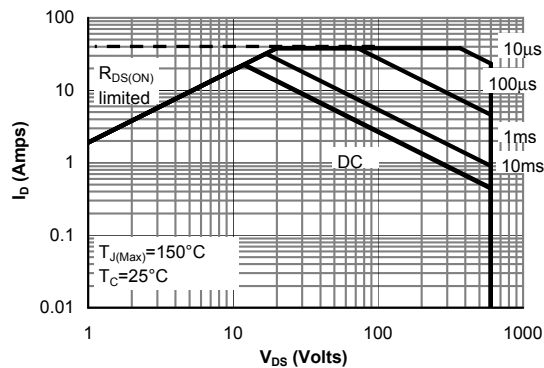
Figure 11: Maximum Forward Biased Safe Operating Area for AOT(B)20S60 (Note F)
