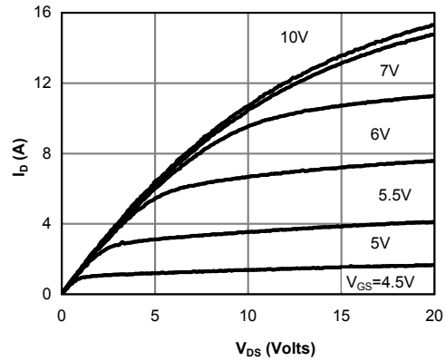
Figure 2: On-Region Characteristics@125°C
