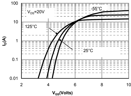
Figure 3: Transfer Characteristics
