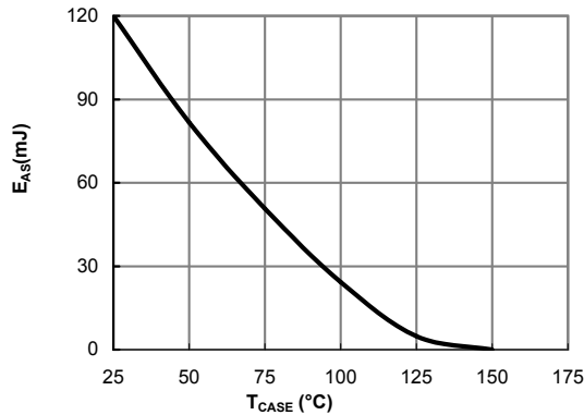
Figure 13: Avalanche energy
