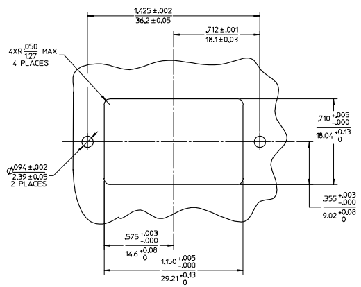
RECOMMENDED MOUNTING PATTERN
