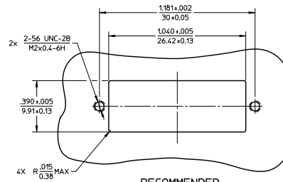
RECOMMENDED MOUNTING PATTERN
