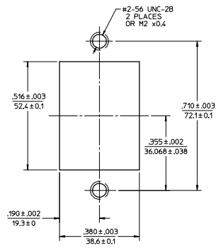
RECOMMENDED MOUNTING CUTOUT FOR .063" THICK PANEL
