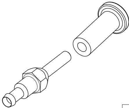
ISOMETRIC VIEW SCALE 8:1
