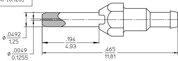
SNAP MATE PLUG, METAL BODY (ZIRCONIA CERAMIC FERRULE)
