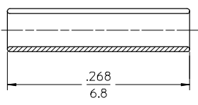
ALIGNMENT SLEEVE (ZIRCONIA CERAMIC)
