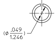
ALIGNMENT SLEEVE (ZIRCONIA CERAMIC)
