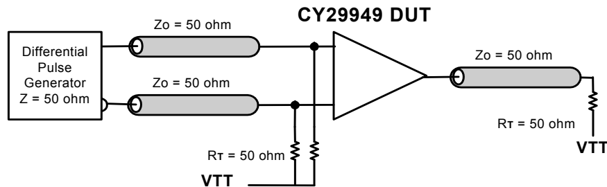
Figure 3. PECL_CLK CY29949 Test Reference for V_{CC} = 3.3V and V_{CC} = 2.5V
