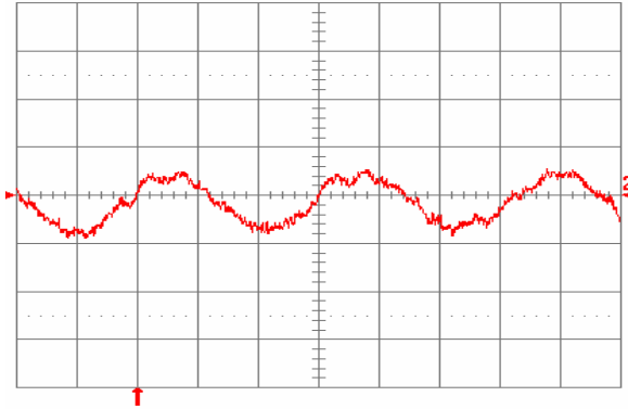
Fig. 17: Input reflected ripple current, i_s (10 mA/div), measured through 10 \mu\text{H} at the source at full rated load current and V_{in} = 56 \text{ V} . Refer to Fig. I for test setup. Time scale: 1 \mu\text{s}/\text{div} .
