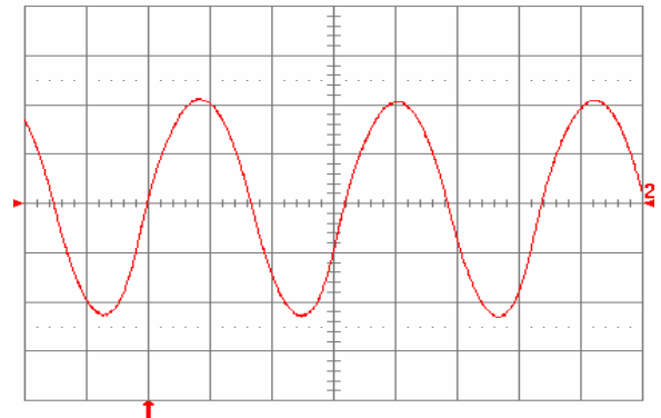
Fig. 20: Input reflected ripple current, i_c (200 mA/div), measured at input terminals at full rated load current and V_{in} = 75 \text{ V} . Refer to Fig. I for test setup. Time scale: 1 \mu\text{s}/\text{div} .
