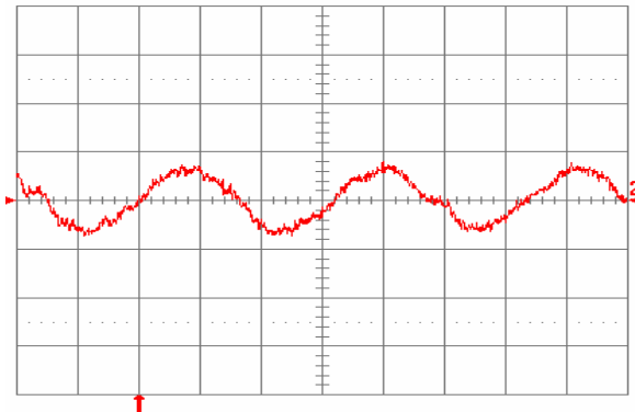
Fig. 19: Input reflected ripple current, i_s (10 mA/div), measured through 10 \mu\text{H} at the source at full rated load current and V_{in} = 75 \text{ V} . Refer to Fig. I for test setup. Time scale: 1 \mu\text{s}/\text{div} .
