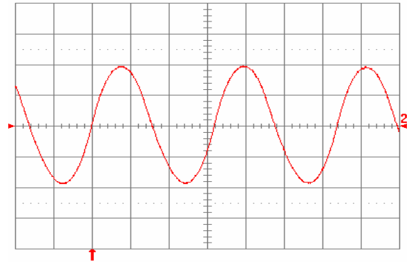
Fig. 18: Input reflected ripple current, i_c (200 mA/div), measured at input terminals at full rated load current and V_{in} = 56 \text{ V} . Refer to Fig. I for test setup. Time scale: 1 \mu\text{s}/\text{div} .
