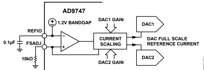
Figure 33. Reference Circuitry
