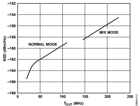
Figure 12. AD9747 NSD vs. f_{OUT} , Single Carrier WCDMA, 245.76 MSPS
