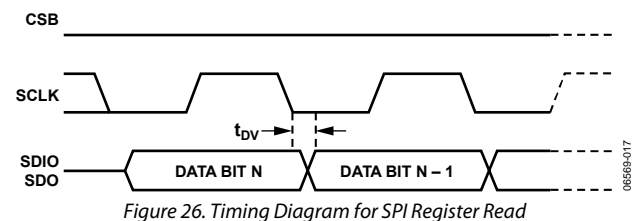
Figure 26. Timing Diagram for SPI Register Read
