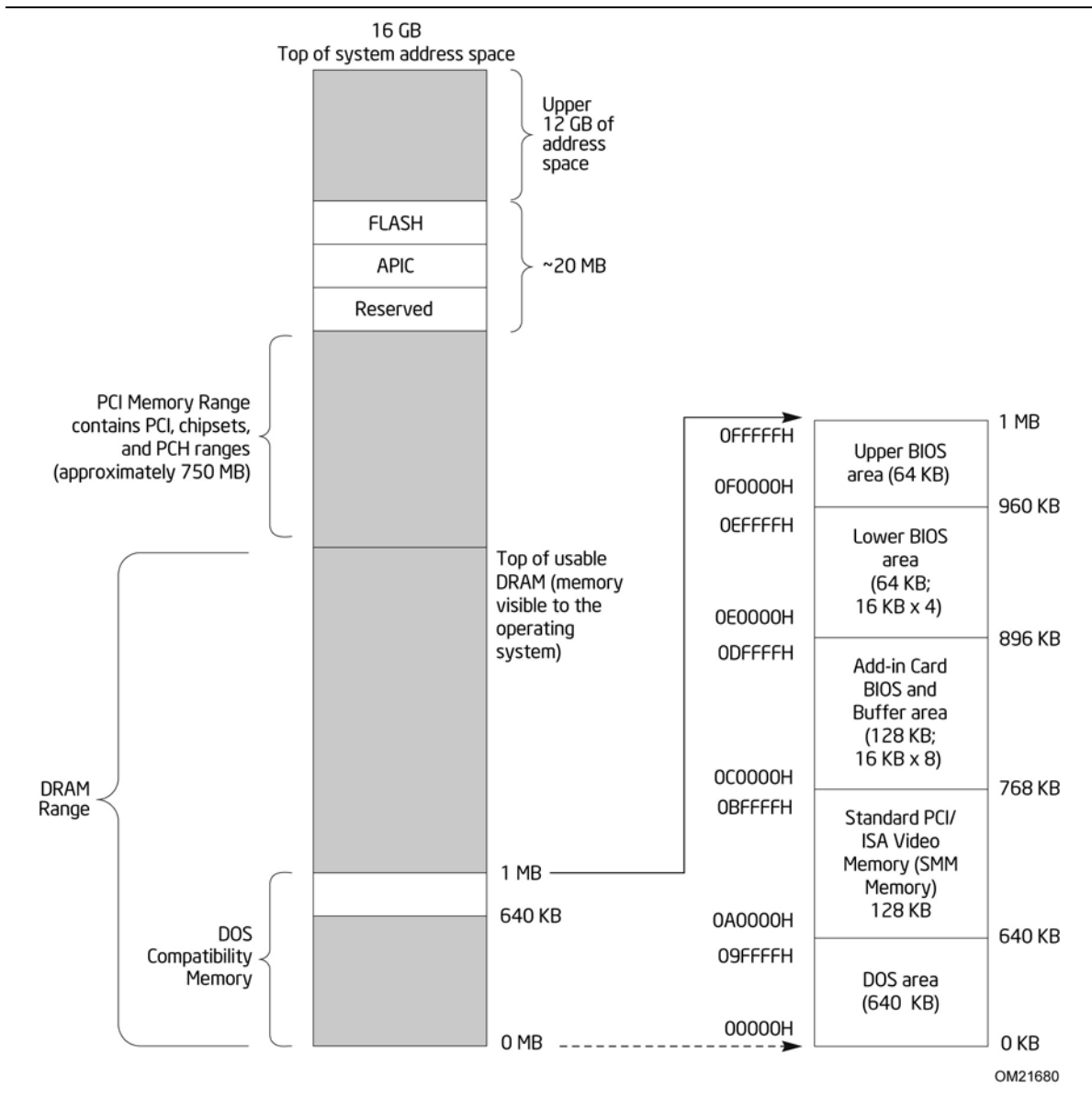
Figure 9. Detailed System Memory Address Map
