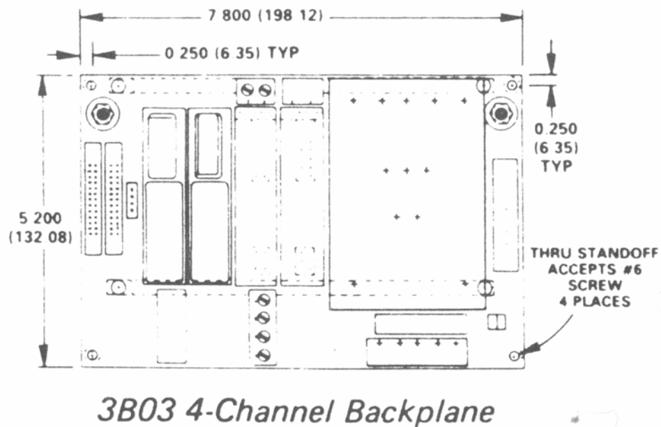
Figure 3 Outline Dimensions
