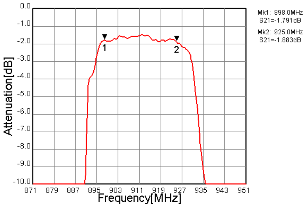
Fig.2 In-band Characteristic (Filter1)
