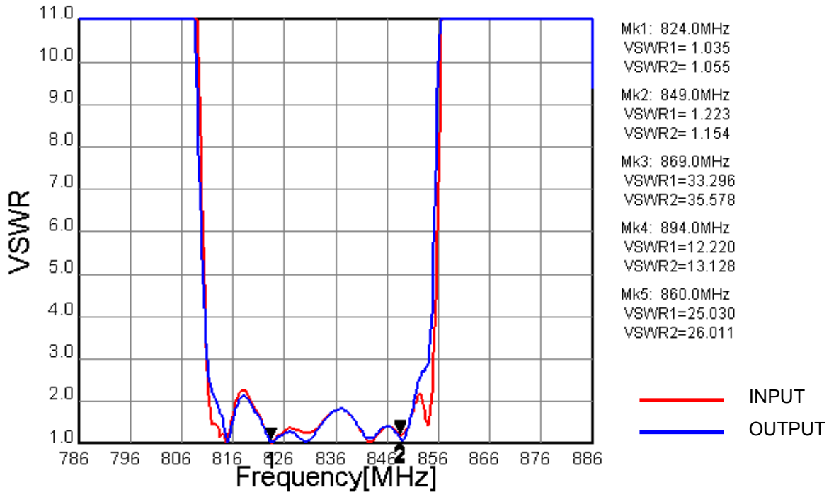
Fig.9 VSWR (Filter2)
