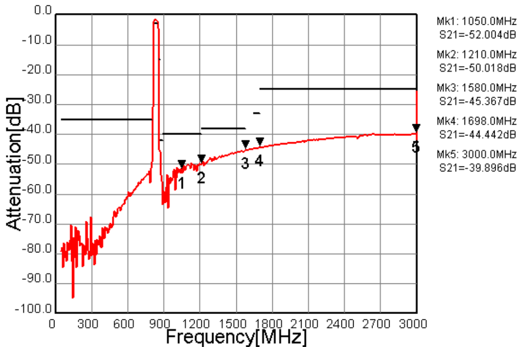
Fig.10 Wide-band Characteristic (Filter2)
