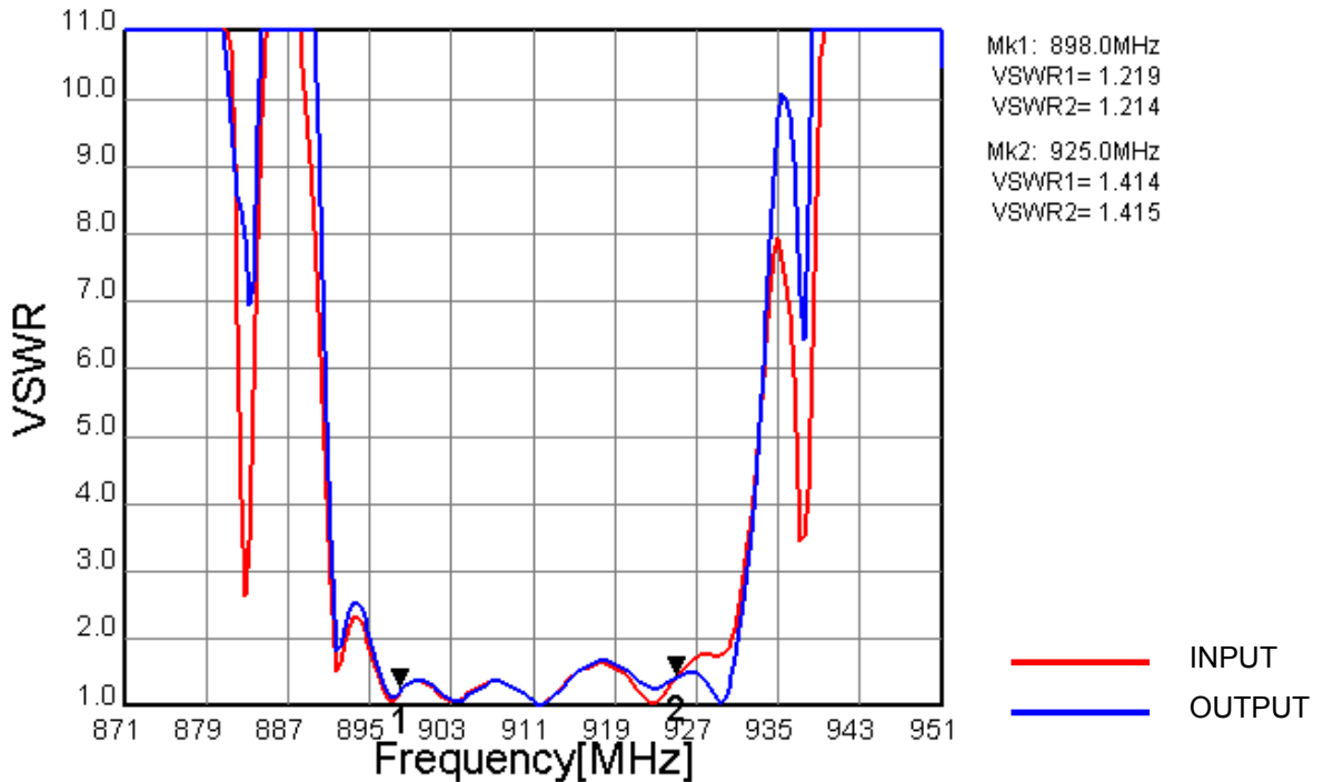
Fig.3 VSWR (Filter1)
