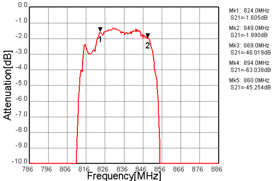
Fig.8 In-band Characteristics (Filter2)
