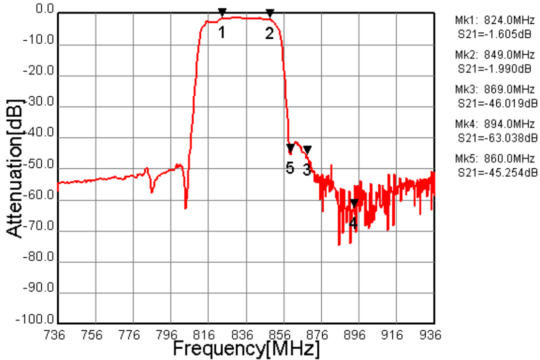
Fig.7 Pass-band Characteristic (Filter2)
