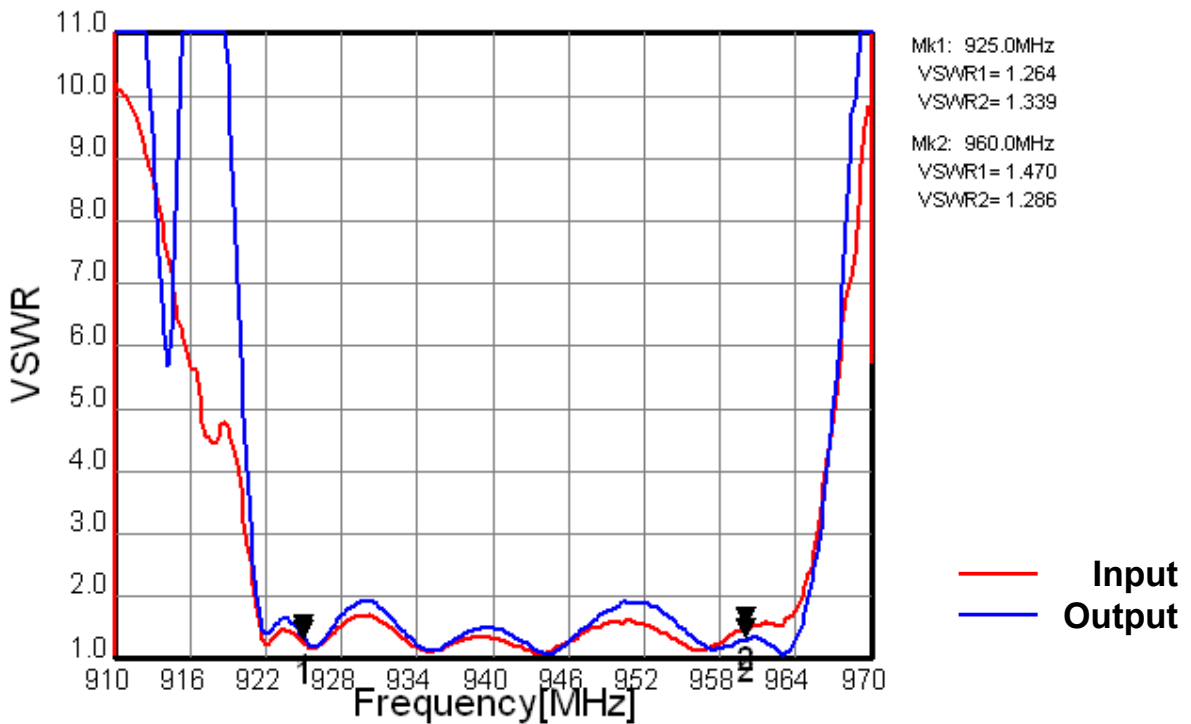
Fig.2 VSWR (Filter1)
