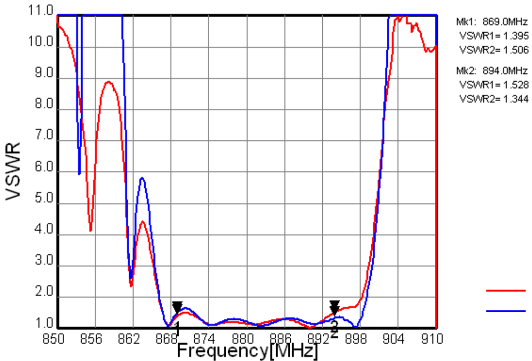
Fig.10 VSWR (Filter2)
