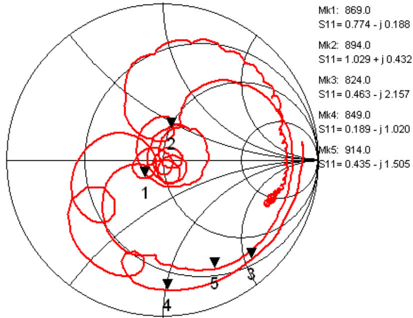
Fig.13 Impedance (SS11) (Filter2)
