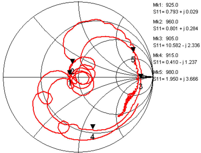
Fig.5 Impedance (SS11) (Filter1)
