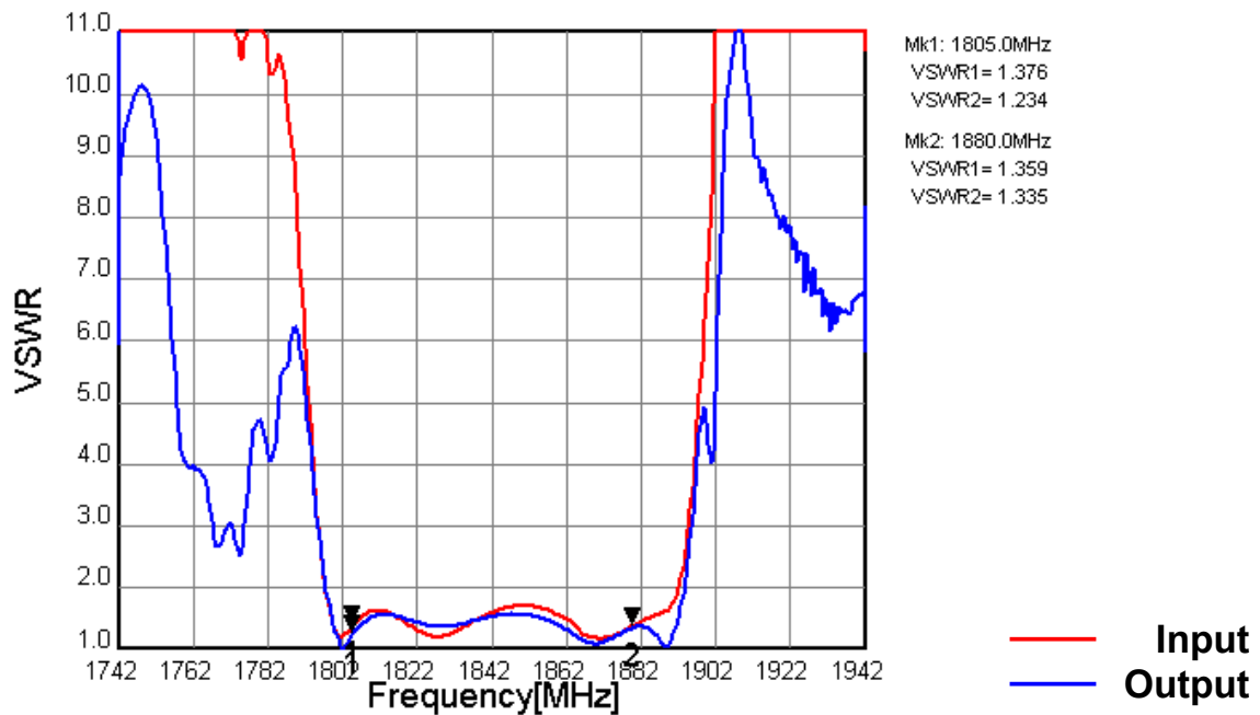
Fig.10 VSWR (Filter2)
