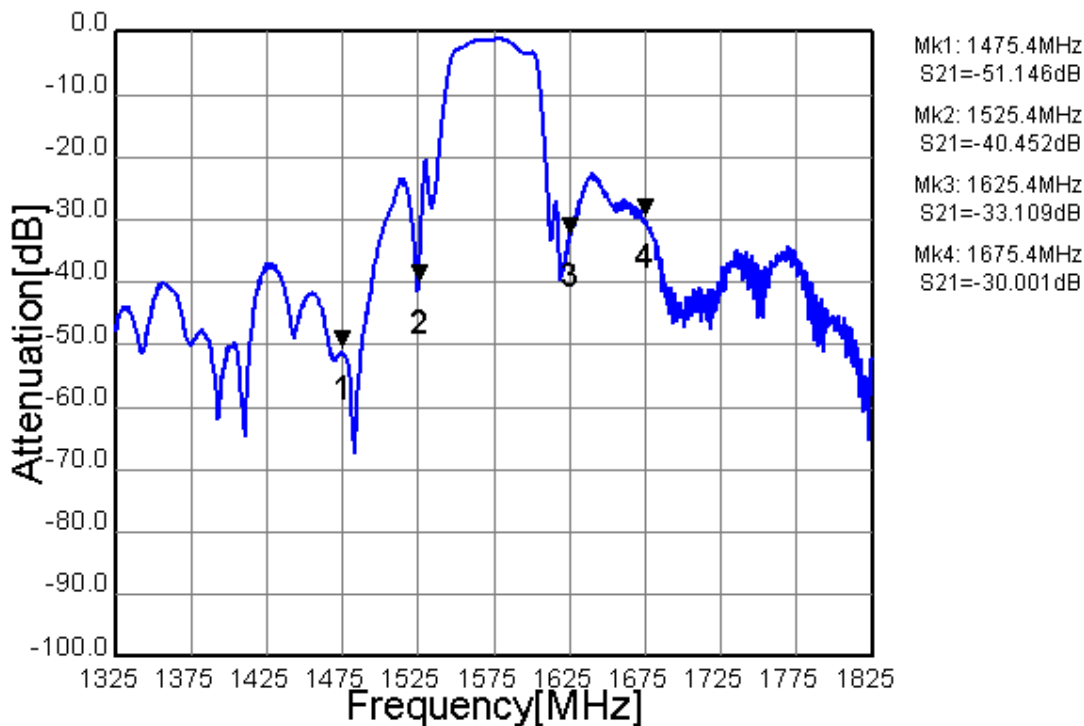
Fig.1 Pass-band Characteristic
