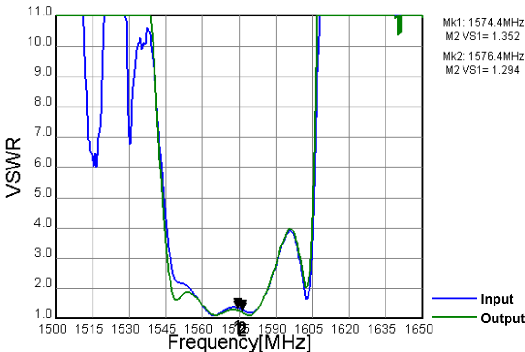
Fig.2 VSWR
