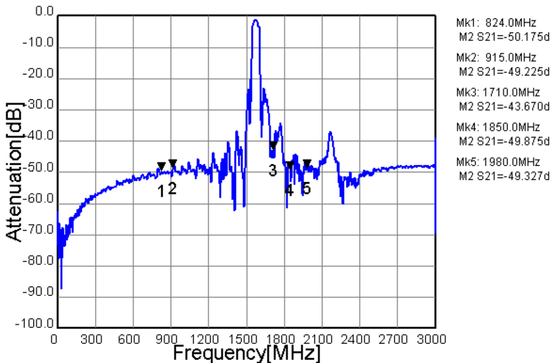
Fig.4 Wide-band Characteristic
