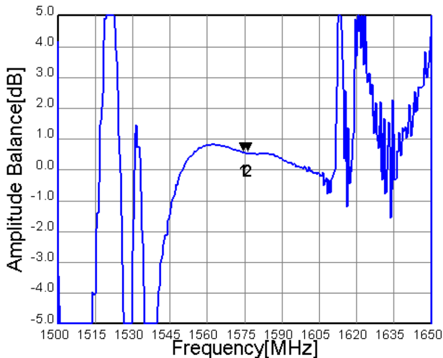
Fig.7 Amplitude Balance
