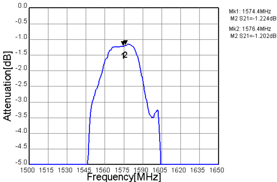
Fig.3 In-band Characteristic
