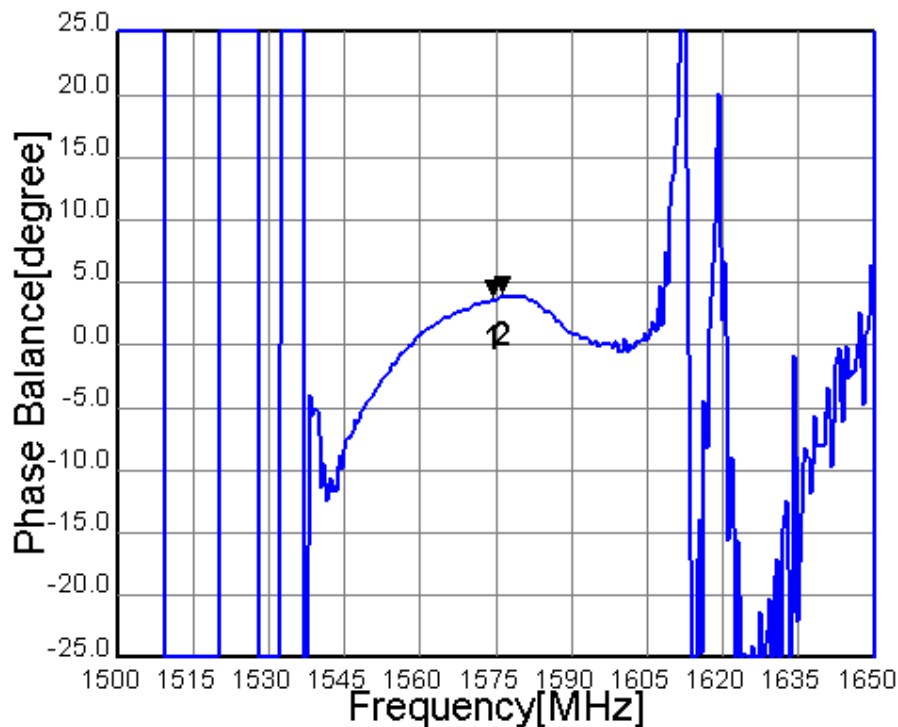
Fig.8 Phase Balance
