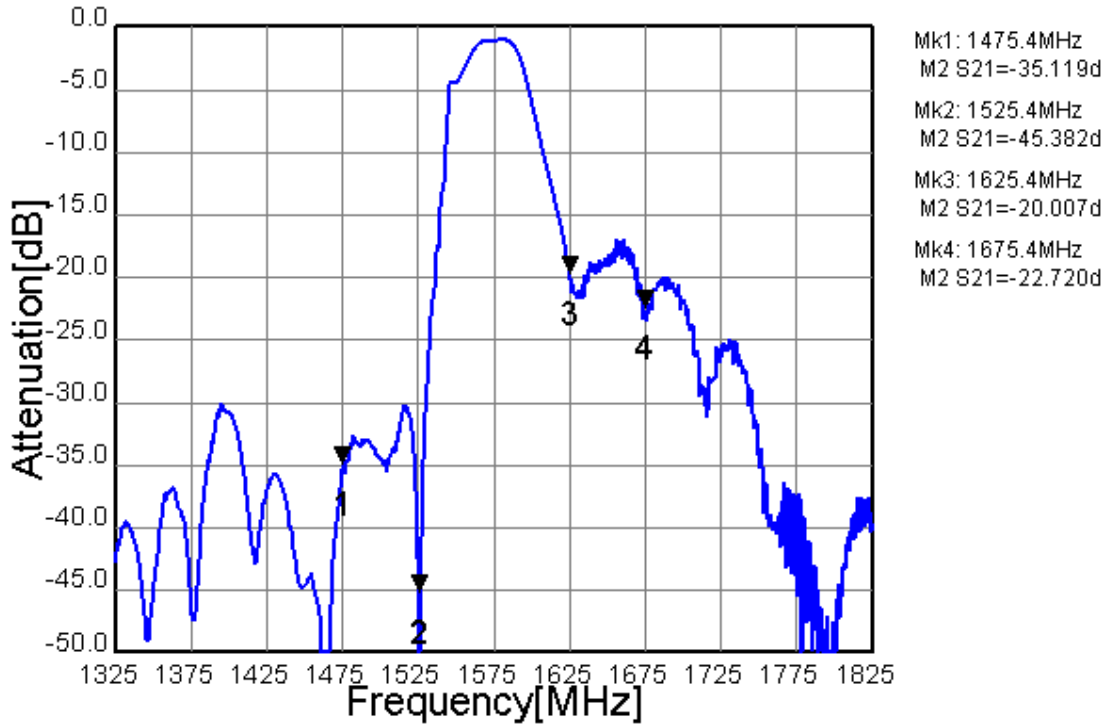
Fig.1 Pass-band Characteristic
