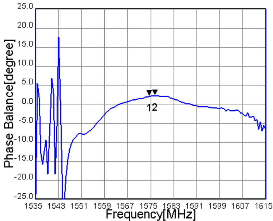
Fig.8 Phase Balance
