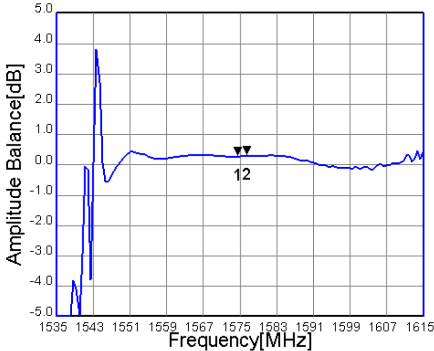
Fig.7 Amplitude Balance
