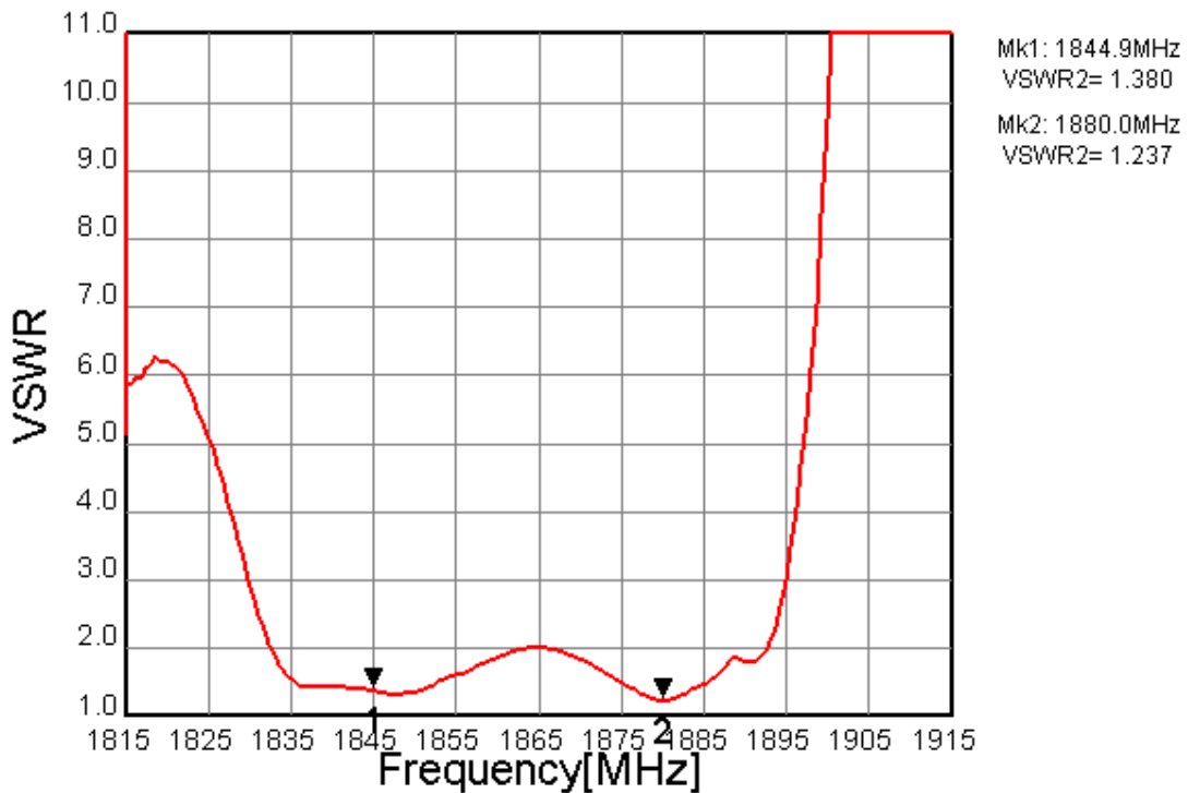
Fig.4 VSWR (bal)
