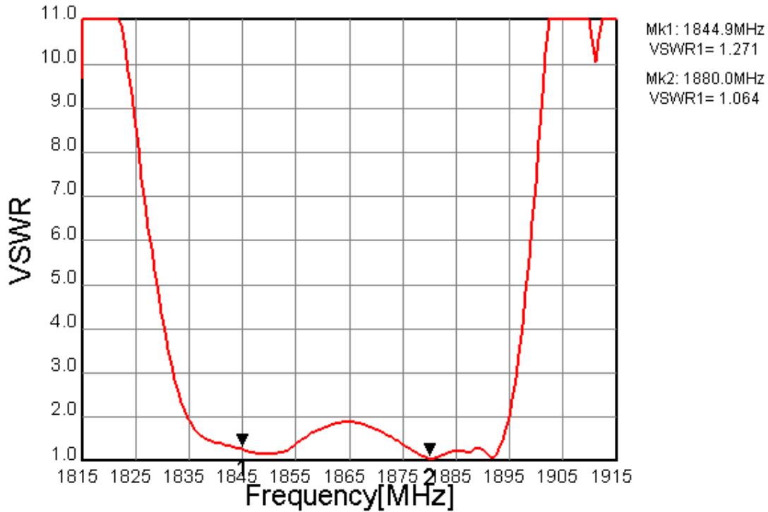
Fig.3 VSWR (unbal)
