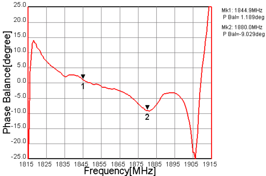
Fig.9 Phase Balance
