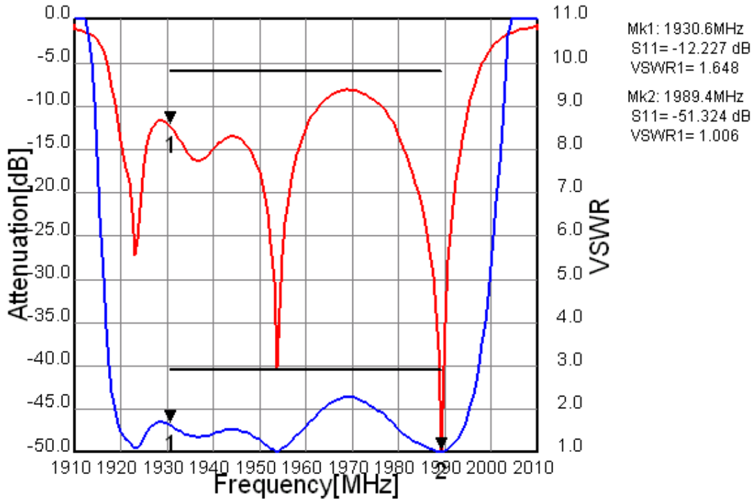
Fig.4 Return Loss and VSWR S11
