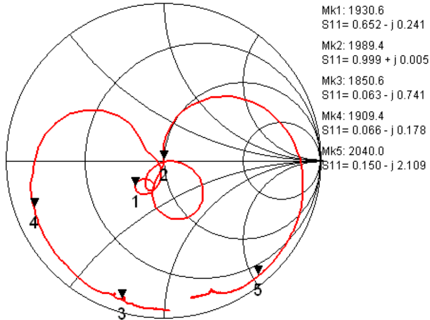
Fig.6 Impedance S11
