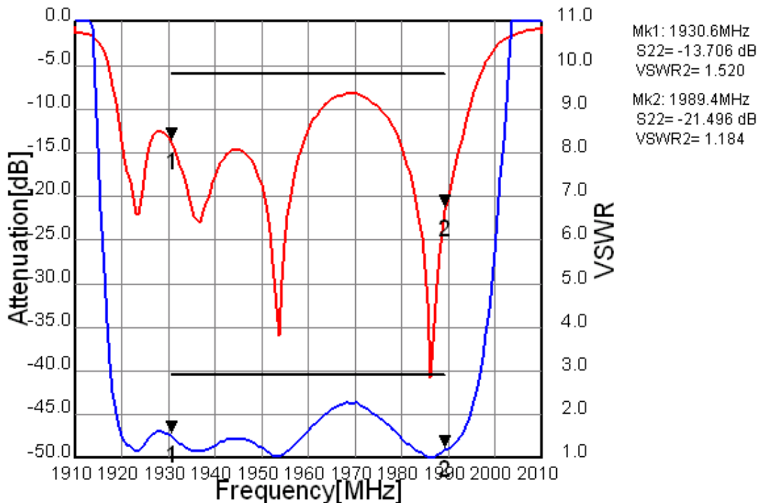
Fig.5 Return Loss and VSWR S22
