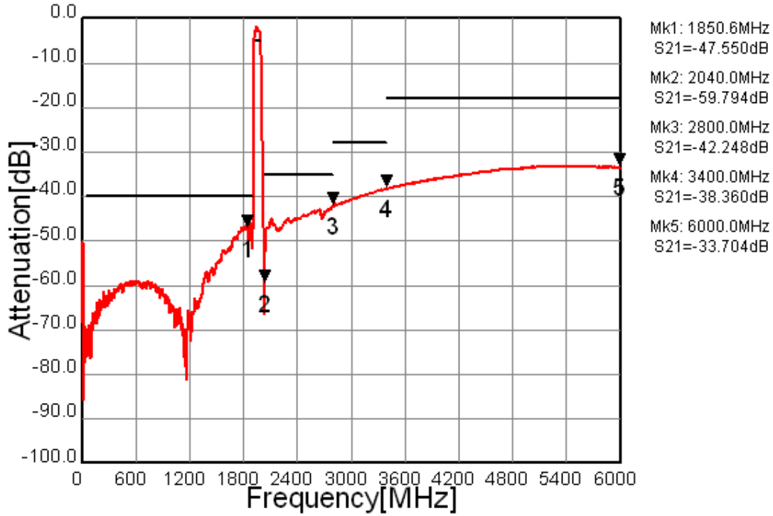
Fig.3 Wide-band Characteristics
