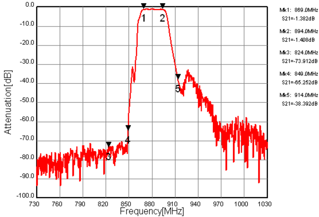
Fig.1 Pass-band Characteristics
