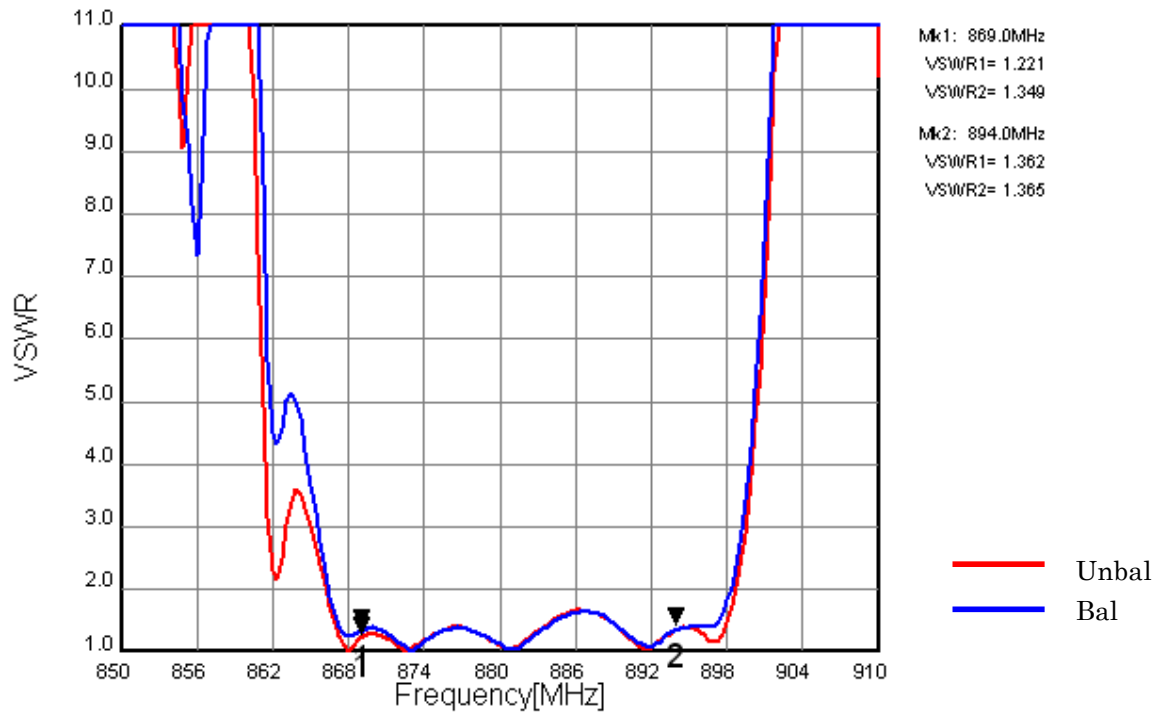
Fig.2 VSWR
