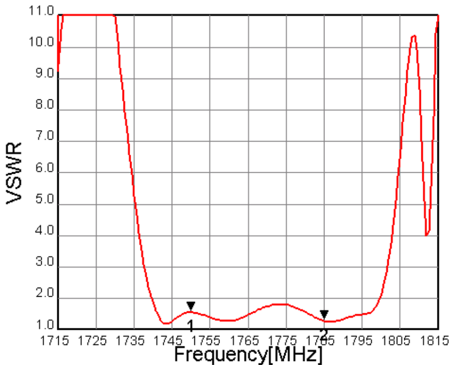
Fig.4 VSWR (S22)
