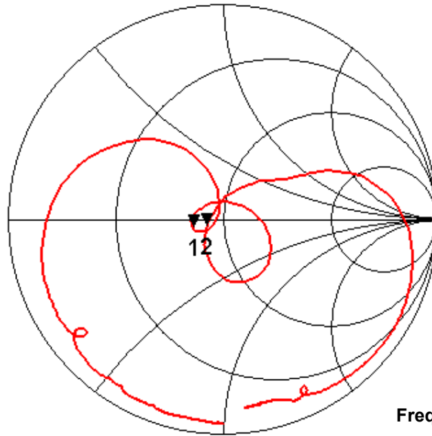
Fig.6 Impedance (Input)
