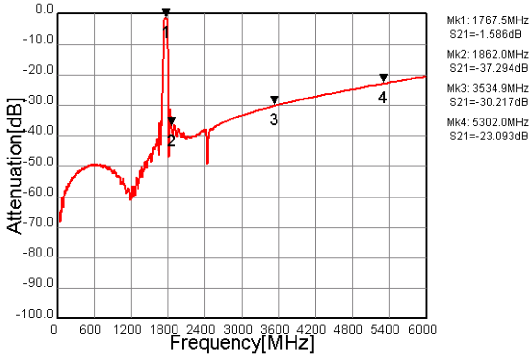
Fig.5 Wide-band Characteristics
