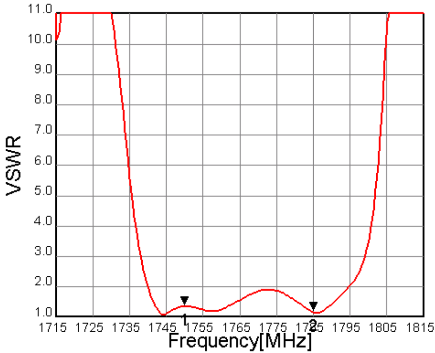
Fig.3 VSWR (S11)
