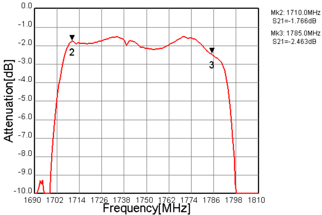
Fig.3 In-band Characteristic
