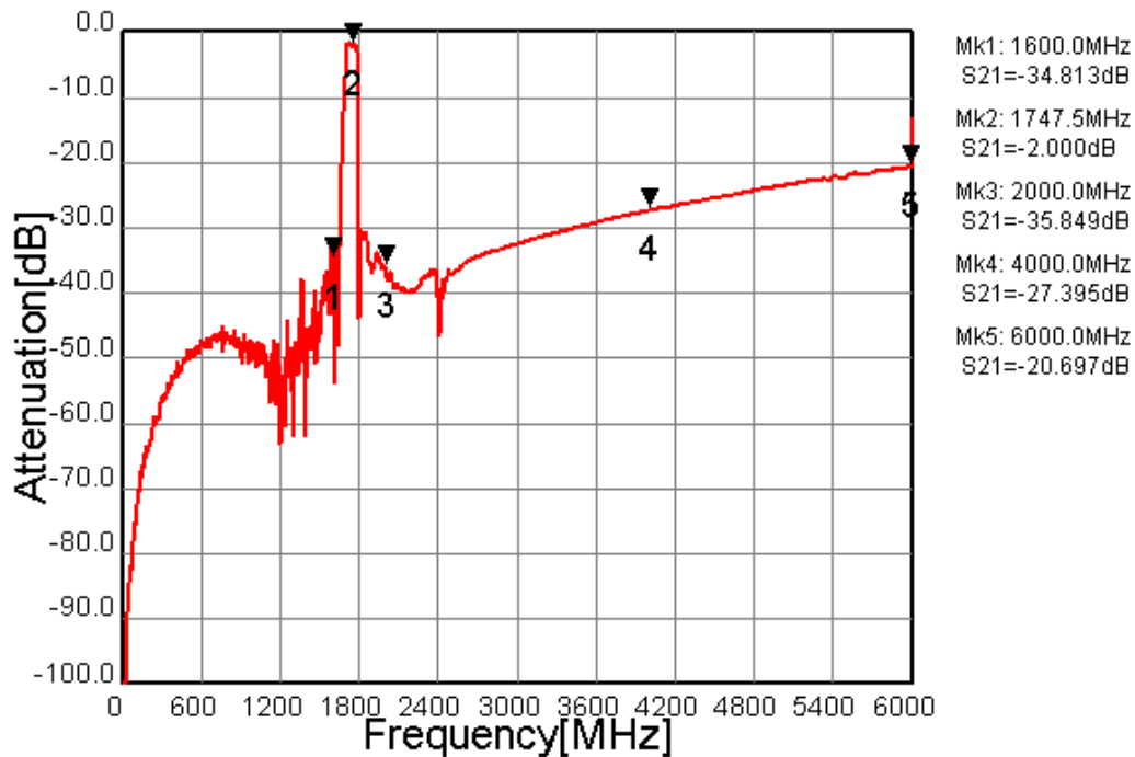
Fig.4 Wide-band Characteristic
