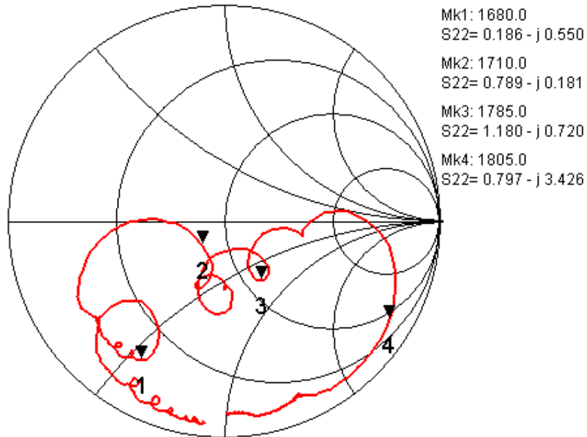
Fig.6 Output Impedance
