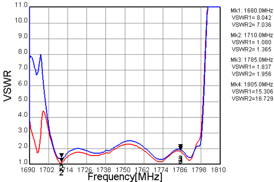
Fig.2 VSWR
