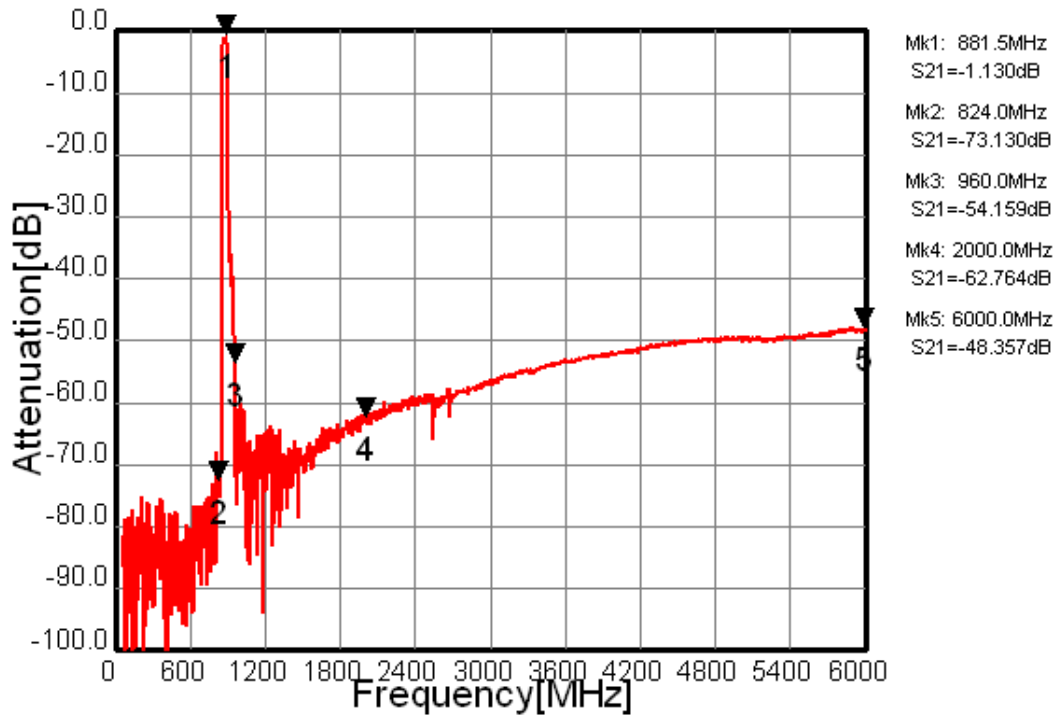
Fig.4 Wide-band Characteristic
