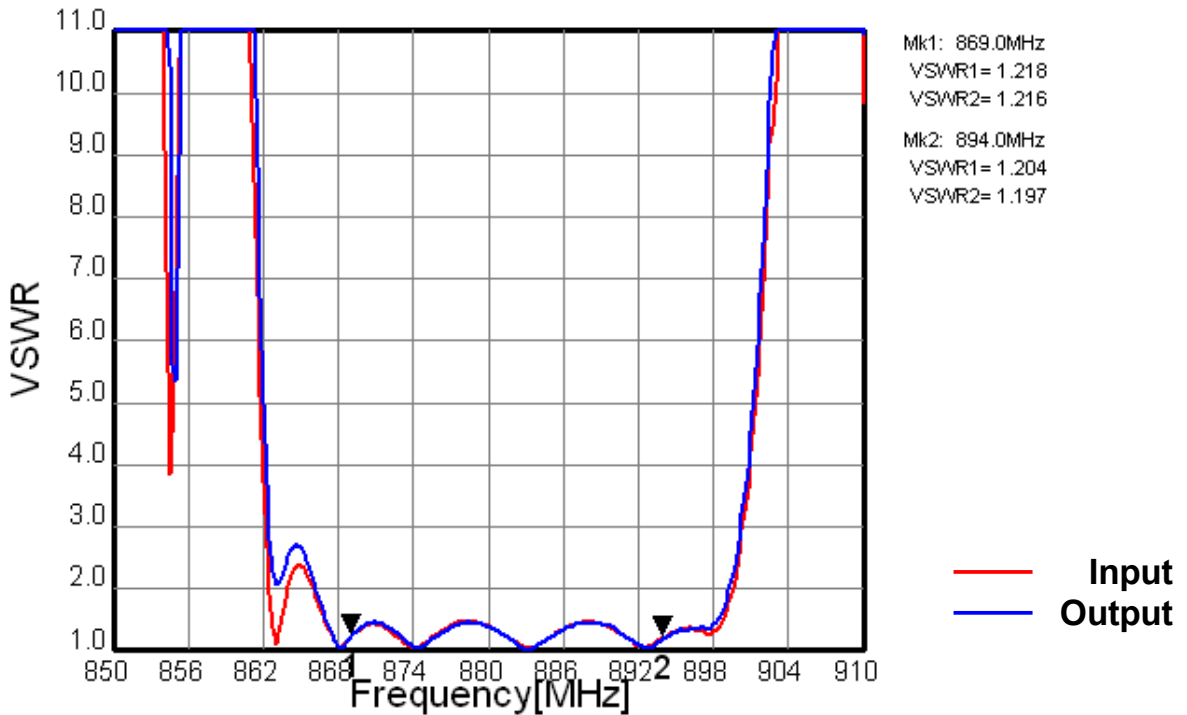
Fig.2 VSWR
