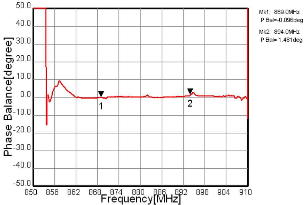
Fig.8 Phase Balance
