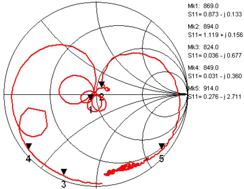
Fig.5 Impedance (S11)
