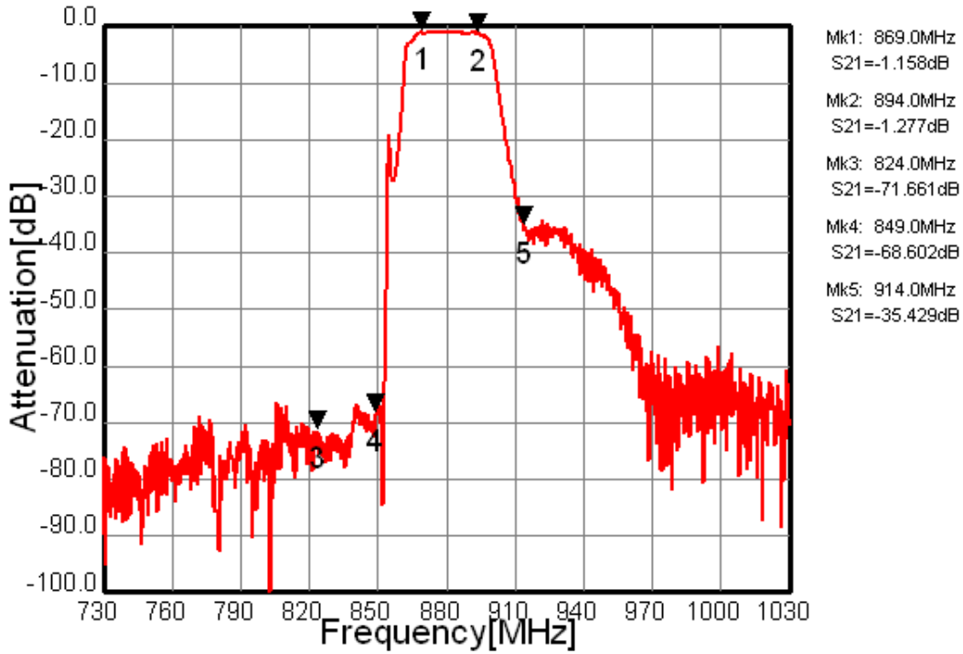
Fig.1 Pass-band Characteristic
