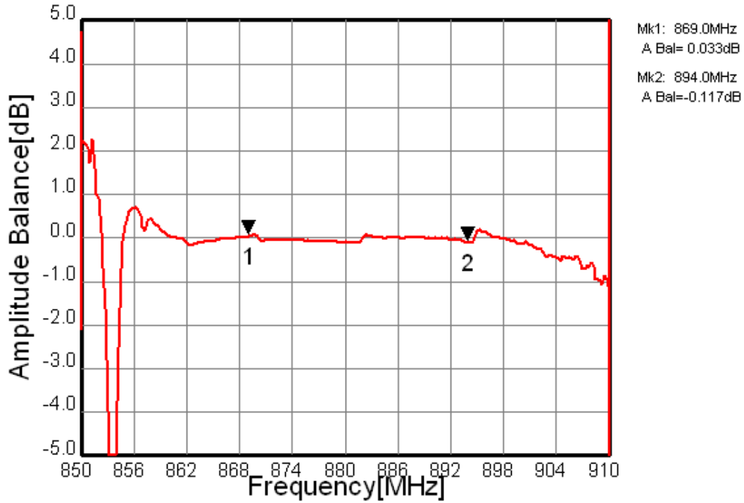
Fig.7 Amplitude Balance
