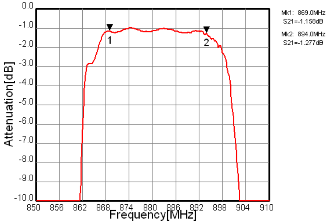
Fig.3 In-band Characteristic
